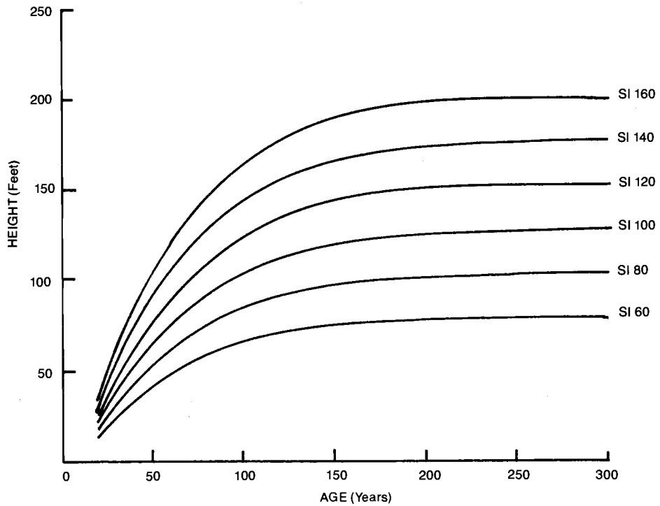
SITE INDEX CURVES FOR WESTERN HEMLOCK FROM SILVICULTURE PRACTICES HANDBOOK (FSH 2409.26d.61.3). INDEX AGE 100.
