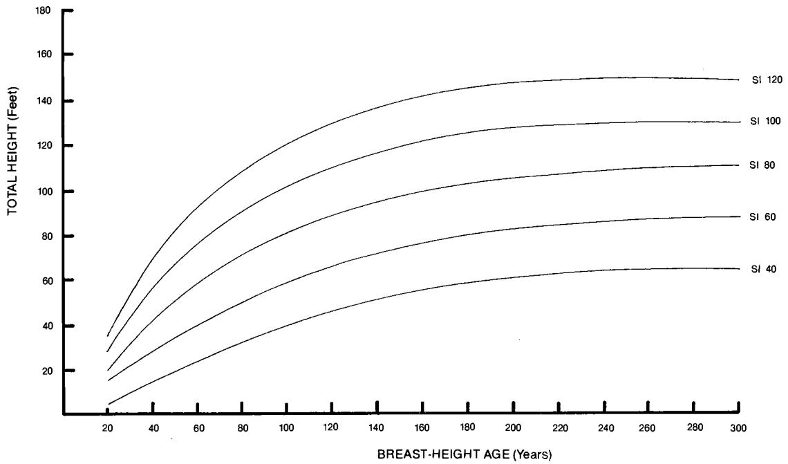
Site Index Curves for Engelmann spruce in Colorado (Alexander, 1967). Index Age 100.
