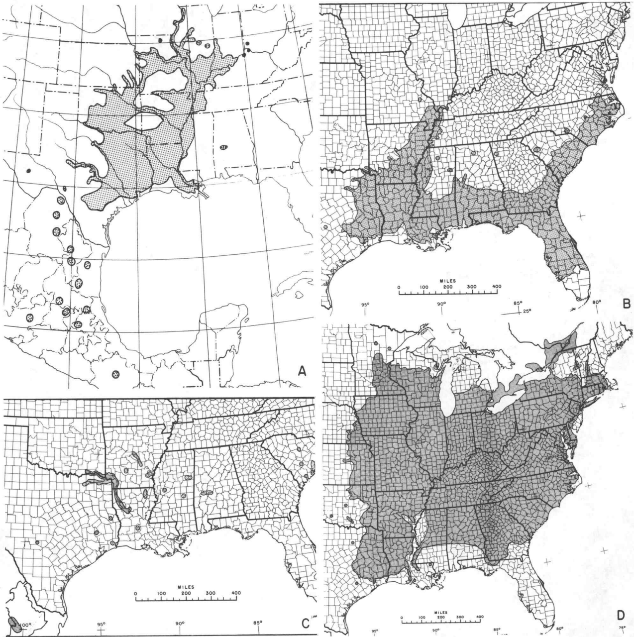
Figure 1.—Natural range of pecan (A), water hickory (B), nutmeg hickory (C), bitternut hickory (D).
