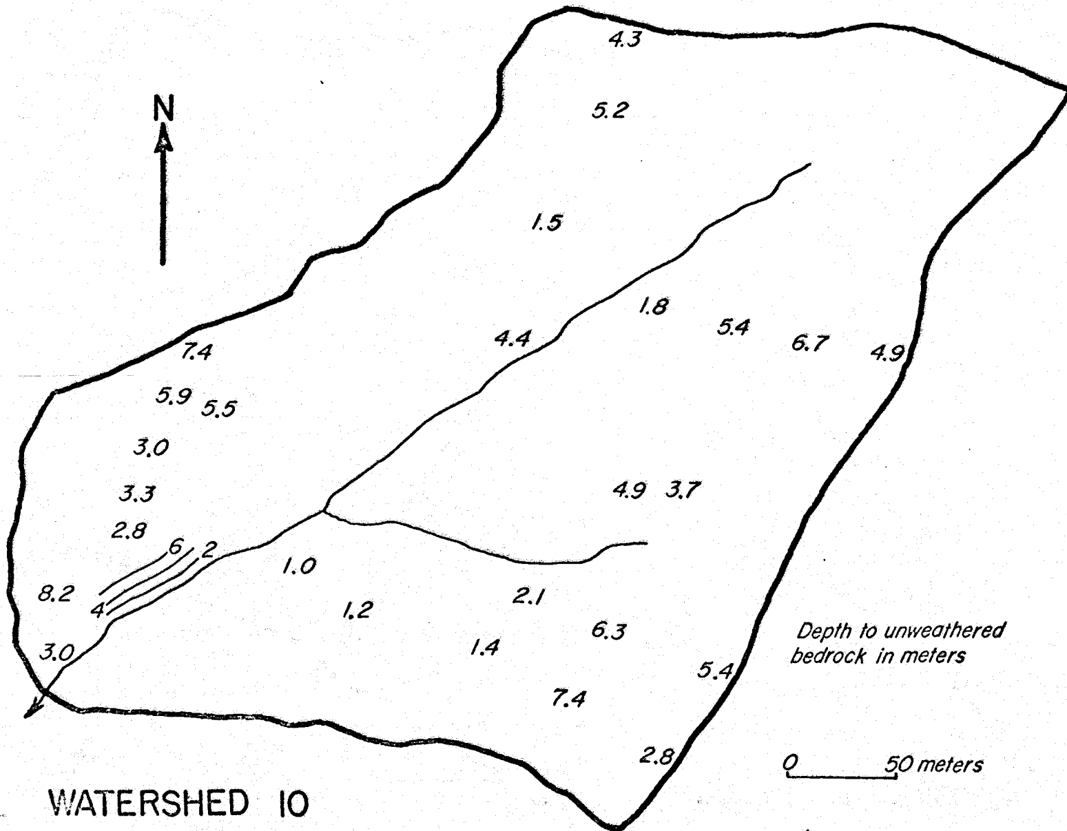
Figure 3. Depth to relatively unweathered bedrock.
