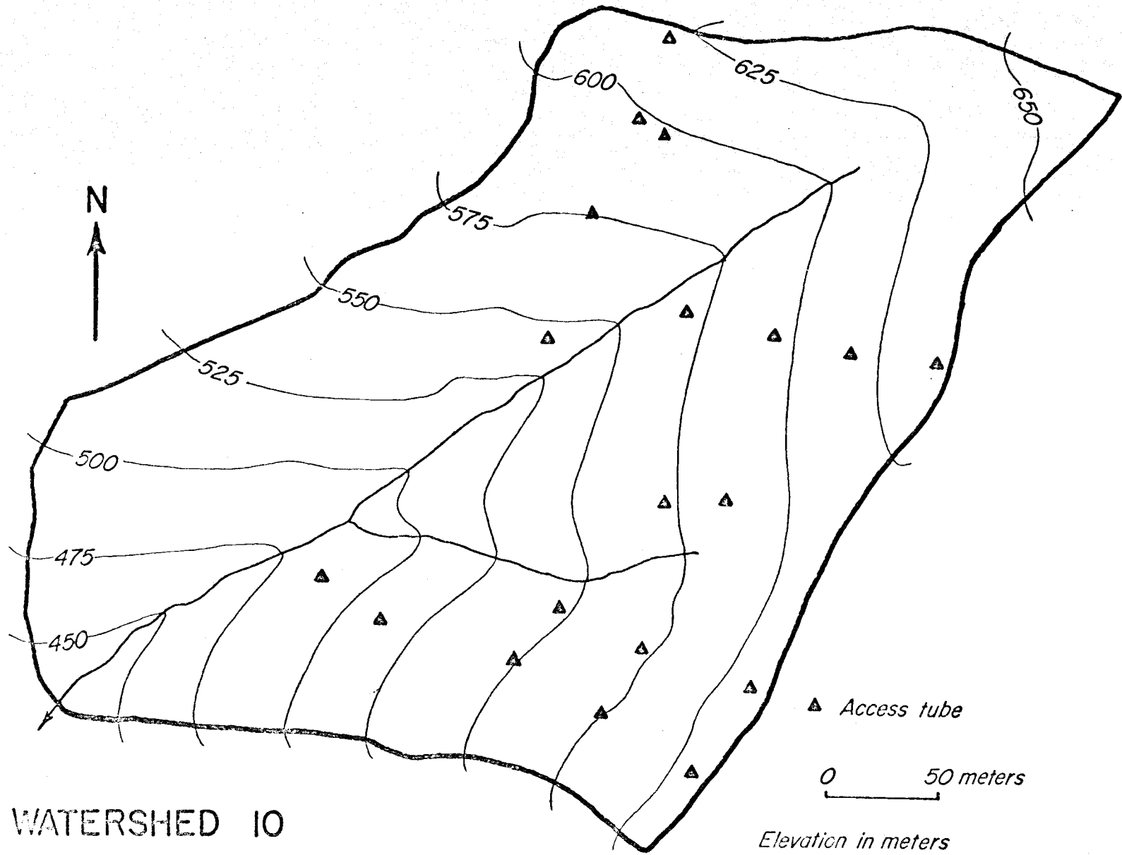
Figure 2. Location of neutron probe access tubes exclusive of those shown in Figure 1.
