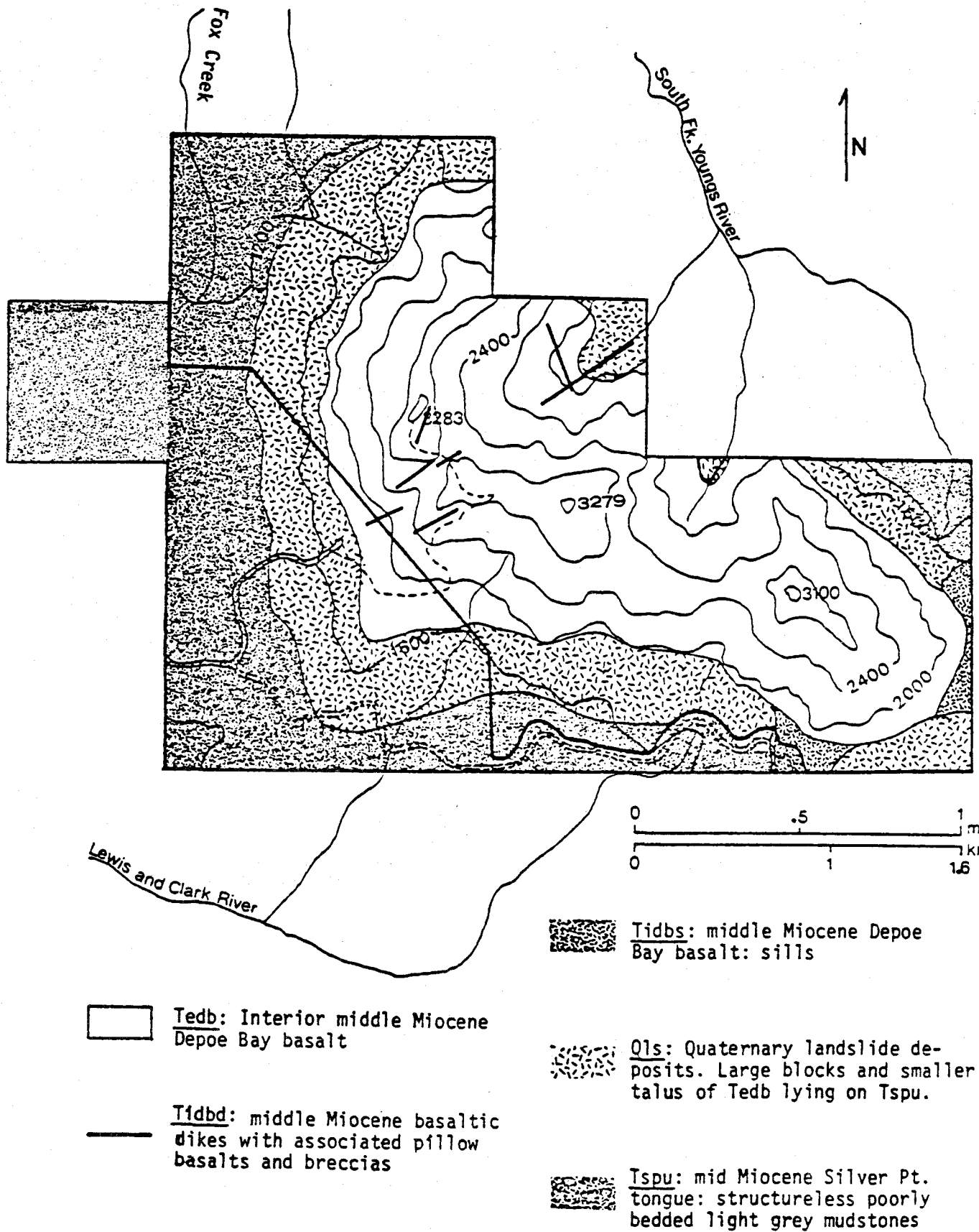
Figure 7. Geology of Saddle Mountain State Park. Adapted from Penoyer (1977)
