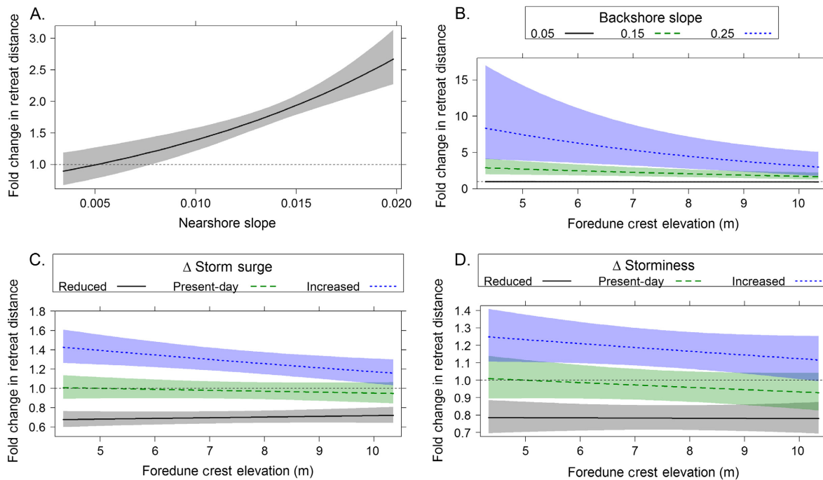
Fig. 5. (A) Main effect of nearshore slope on foredune retreat distance. Interactive effect of (B) backshore slope \times d_{\text{crest}} elevation, (C) \Delta storm surge \times d_{\text{crest}} elevation, and (D) \Delta storminess \times d_{\text{crest}} elevation on foredune retreat distance. Fold change in foredune retreat distance measures the relative amount of retreat for foredunes under different conditions as compared to a reference condition (conditions with a predicted 1 \times -fold change). Bands indicate confidence intervals.
