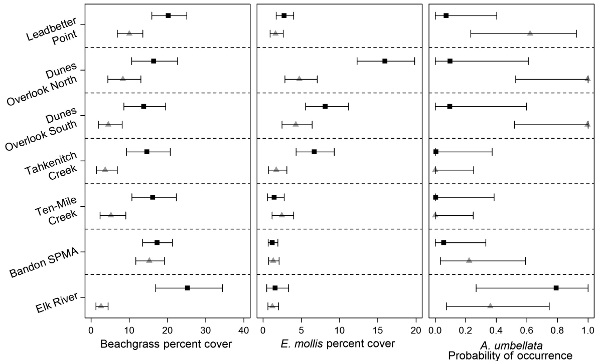
Fig. 8. (A) Beachgrass percent cover; (B) native dune grass percent cover; and (C) pink sand verbena probability of occurrence at beachgrass removal (gray triangles) and reference (black squares) areas at seven habitat restoration area sites (Fig. 1; Appendix S1: Table S1). Points indicate median posterior estimates; error bars indicate 95% posterior intervals.
