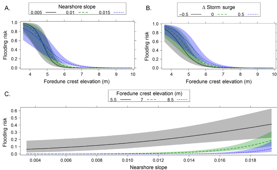
Fig. 4. Interactive effect of (A, C) nearshore slope \times d_{crest} elevation and (B) \Delta storm surge \times d_{crest} elevation on absolute flooding risk. Bands indicate confidence intervals.
