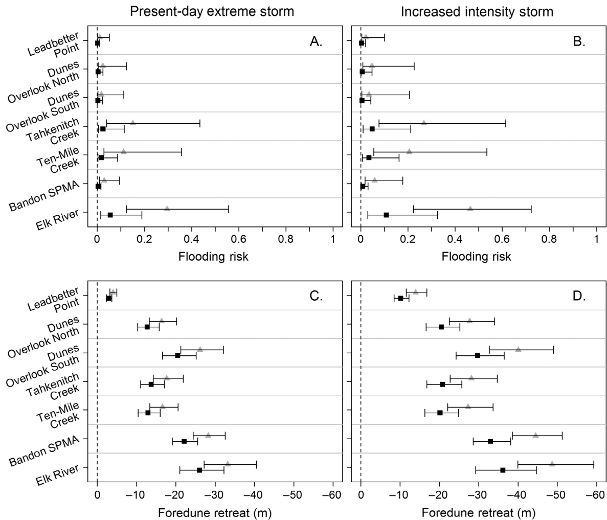
Fig. 6. (A, B) Flooding risk (probability of flooding) at beachgrass removal (gray triangles) and reference (black squares) sites under (A) a present-day extreme storm scenario and (B) an increased wave intensity and surge extreme storm scenario. (C, D) Predicted foredune retreat at beachgrass removal and reference areas under (C) a present-day extreme storm scenario and (D) an increased wave intensity and surge extreme storm scenario. Error bars indicate 95% confidence interval.
