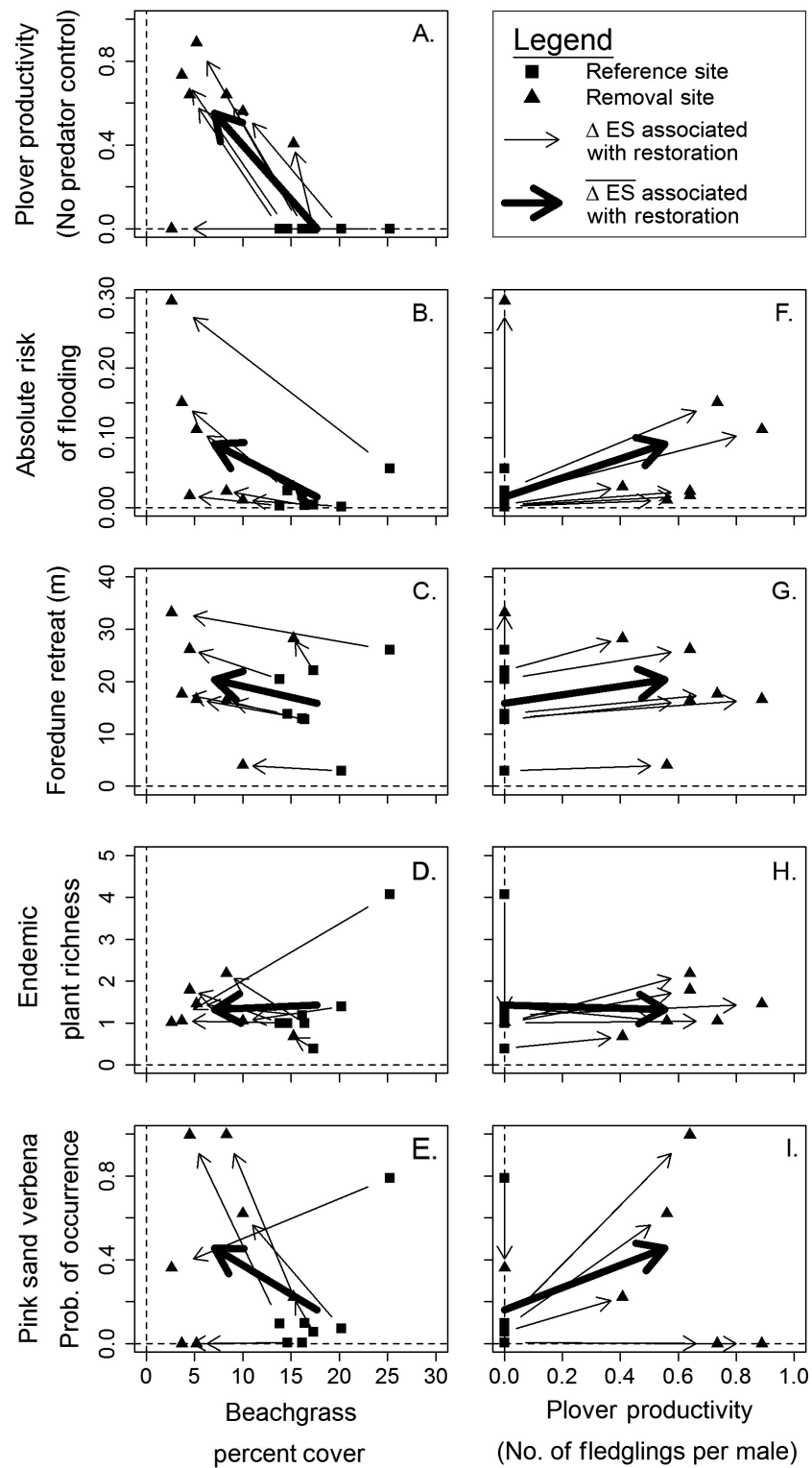
Fig. 9. (A–E) Comparison of ecosystem service (ES) metrics with beachgrass percent cover at paired beachgrass removal (black triangles) and reference (black squares) areas at seven habitat restoration area sites (Fig. 1;
