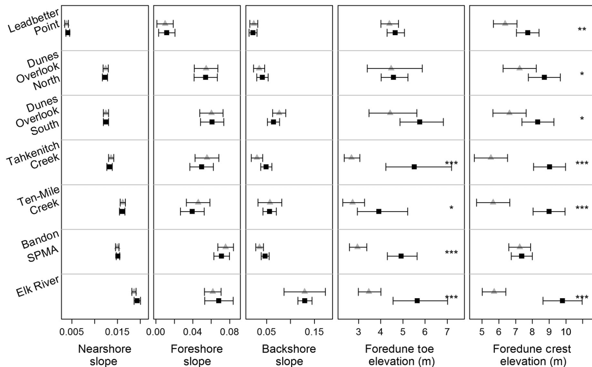
Fig. 3. Dune geomorphology at beachgrass removal (gray triangles) and reference (black squares) areas at seven habitat restoration area (HRA) sites (Fig. 1; Appendix S1: Table S1). Error bars indicate 95% confidence intervals. Asterisks indicate significant difference within HRA sites: * P < 0.05 , ** P < 0.01 , *** P < 0.001 .
