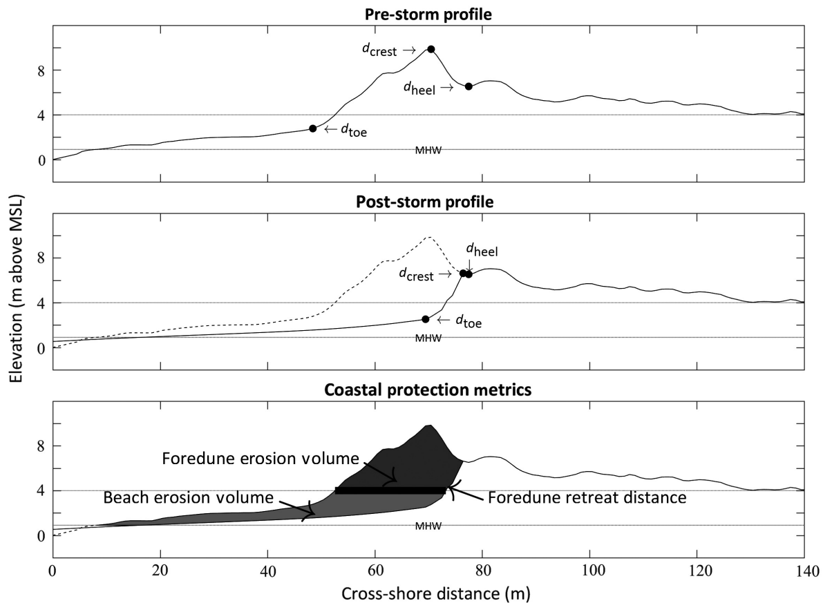
Fig. 2. An example of pre- and post-storm cross-shore profiles at a Ten-Mile Creek habitat restoration area (HRA). Foredune toe ( d_{\text{toe}} ), foredune crest ( d_{\text{crest}} ), and foredune heel ( d_{\text{heel}} ) positions are indicated for both the pre-storm and post-storm profiles. Shading indicates the cross-sectional area eroded during the simulated storm (dark gray = foredune erosion volume; medium gray = beach erosion volume; black line = foredune retreat distance).
