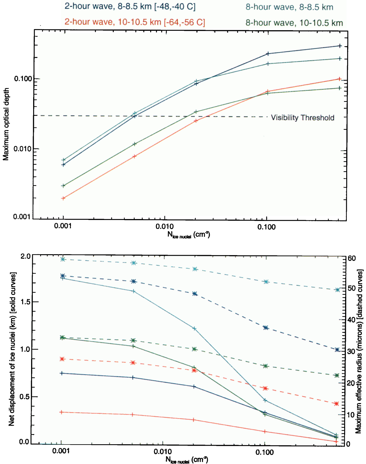
Plate 5. (top) Peak cloud optical depth plotted versus the initial IN number density. (bottom) Effective vertical displacement of ice nuclei by cloud scavenging (solid curves) and maximum ice crystal effective radius (dashed curves) versus IN number density. The different curves correspond to simulations with the high humidity layer at different heights and different timescales for the imposed vertical motion.
