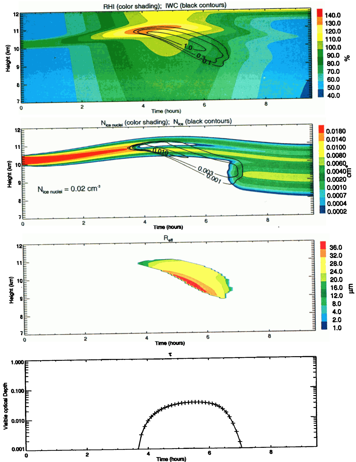
Plate 4. Results from the baseline simulation with an ice number density of 0.02 \text{ cm}^{-3} . Panels (from top to bottom): relative humidity with respect to ice (color shading) and ice water content (milligrams per cubic meter, black contours) versus time and height; IN number density (color shading) and ice crystal number density (black contours, \text{cm}^{-3} ); ice crystal effective radius; zenith visible cloud optical depth versus time.
