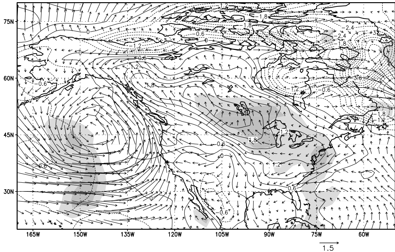
(b) -NAO/EI Nino (state 3)
