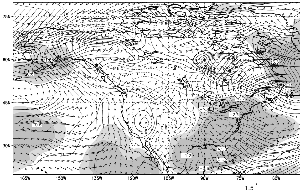
Figure 11. (a–d) Same as Figure 10 but for SAT (contour) and surface wind anomalies. The intervals of SAT anomalies are 0.3°C.
