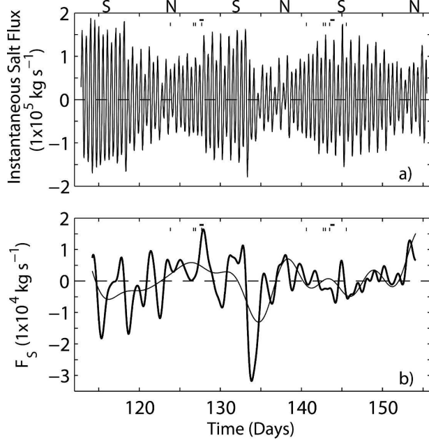
FIG. 7. (a) Instantaneous salt flux and (b) tidally averaged salt flux \mathcal{F}_S at the cross-channel mooring array (thick line). The thin line shows the total salt flux, low-pass filtered to removed fluctuations with periods shorter than 5 days. Note that the y-axis scales are different for the two panels. A negative value indicates an oceanward salt flux.
