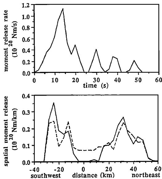
Fig. 3. a) Seismic moment release rate as a function of time (source time function) for best point source PS (Table 1). b) Seismic moment release along the fault length for the bilaterally propagating source BS2 (solid line) (Table 1) and a bilateral rupture model with additional slip in the epicentral region during later stages of the rupture (dashed line). Both models fit the data equally well.
