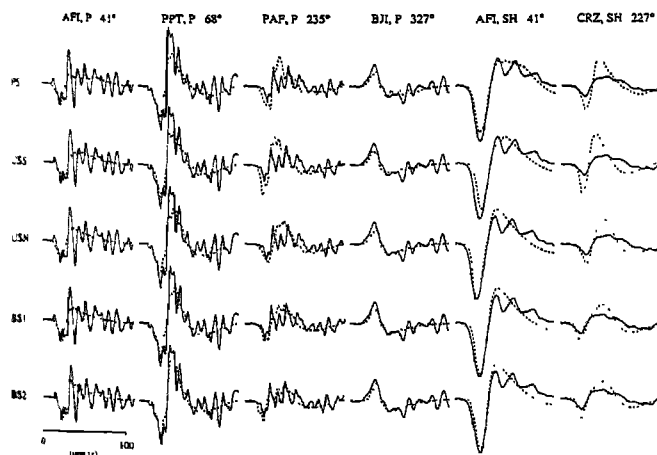
Fig. 4. Comparison of P and SH waveforms for different models listed in Table 1. Number next to the station code is the azimuth from the source.
