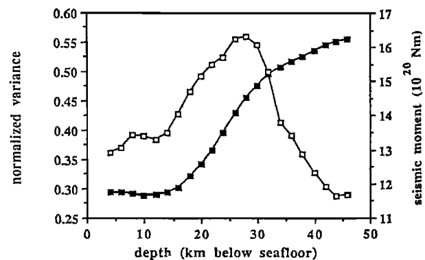
Fig. 2. Residual variance (filled squares) and seismic moment (open squares) as a function of centroid depth.
