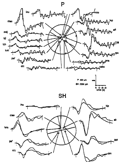
Fig. 5. Observed (solid) and theoretical (dashed) P and SH waves for the model BS2 in Table 1. Fault plane solution for the sum of the two subevents is shown at the center of the figure. Seismogram amplitudes are normalized to an epicentral distance of 40^\circ .
