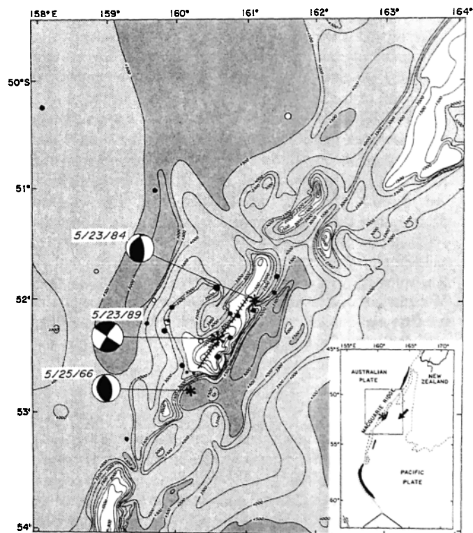
Fig. 1. Bathymetric map of the epicentral area. Epicentral locations and source mechanisms of the 1989 earthquake (large star) and two thrust events 25 May 1966, M=6.5 and 23 May 1984, M=5.9 are shown. The first week of aftershocks is indicated by solid circles and those recorded since then until December 1989 by open circles (only aftershocks recorded by 20 or more stations are depicted; PDE data). The region in which 80% of the moment release occurred during the 1989 event is dashed. Bathymetry is shown by 500 m contours. Dark shading indicates areas deeper than 4500 m, light shading 2000-4500 m, and white areas are shallower than 2000 m. Topographic segmentation of the ridge in the epicentral area is apparent. The insert shows a tectonic overview. The arrow indicates the relative plate motion between the Pacific and Australian plates according to the NUVEL-1 model (DeMets et al., 1990). 1800 m depth contours are dashed, depths greater than 4800 m are shaded.
