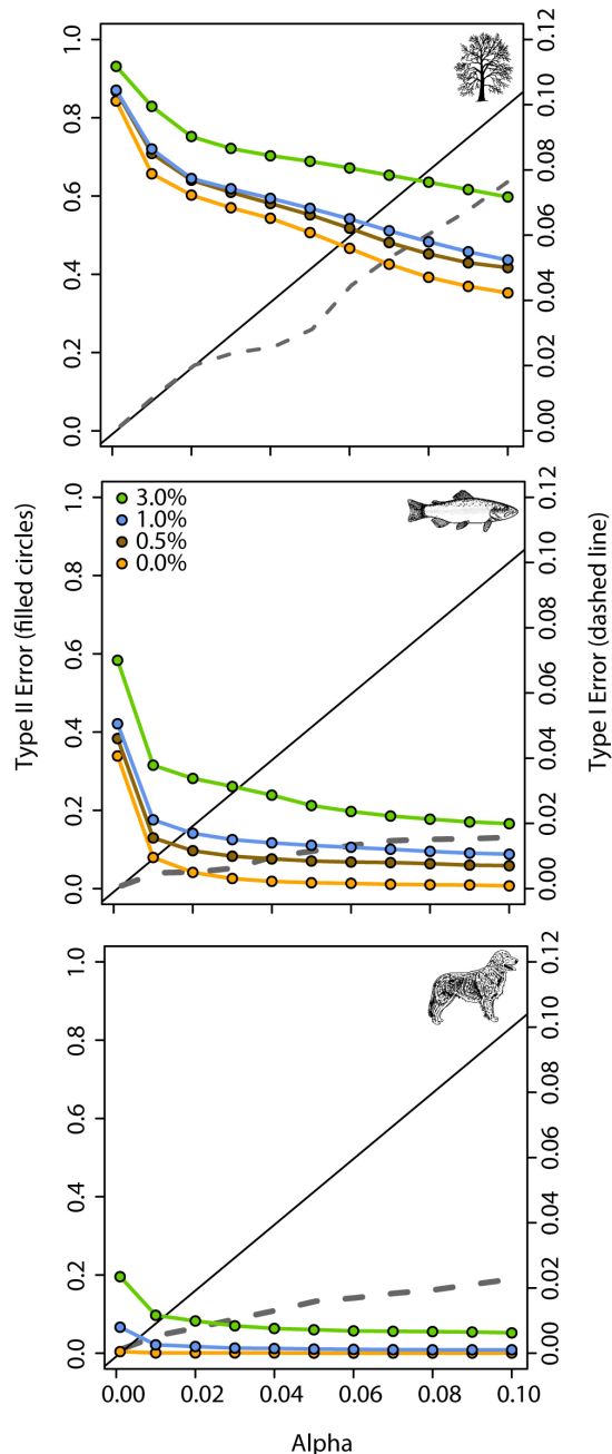
Fig. 2. The relationship between alpha and the type I and II error rate. Genotyping error rates were varied from 0 to 3%. Each panel represents 100 test data sets with 100 adults, 100 juveniles and 50 true parent-offspring pairs. The maximum observed type I error was plotted as a dashed gray line. Type I error is consistently at or below \alpha (solid line), indicating that our method is conservative and does not produce an excess of false positive parent-offspring pairs. For the steelhead and Labrador retriever datasets, an increase in alpha beyond 0.05 recovers few additional true parent-offspring pairs. The lowest alpha value plotted is 0.001 and the 0.5% genotyping error was omitted from the retriever data set for visual clarity. See figure S1 to view these results on a logarithmic scale.
