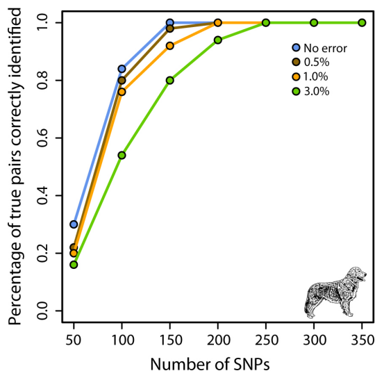
Fig. 3. Relationship between the number of used SNPs and the percentage of true parent-offspring pairs that were correctly identified in the retriever data sets. Genotyping error rates were varied from 0 to 3%, and all parent-offspring pairs were correctly identified with 250 SNPs. Notice that small amounts of error do not substantially affect the assignment rate with intermediate numbers of loci.
