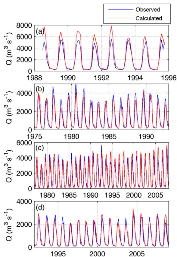
Figure 6. Observed and predicted hydrographs for the (a) Copper (USGS 15215000), (b) Susitna (USGS 15294350), (c) Stikine (USGS 15024800), and (d) Alek (USGS 15129000) Rivers.
