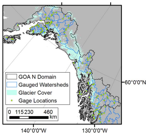
Figure 11. Glacier coverage from the Randolph glacier inventory (v.3.2) [Pfeffer et al. , 2014], gauged watersheds, gaging stations, and the GOA N domain.
