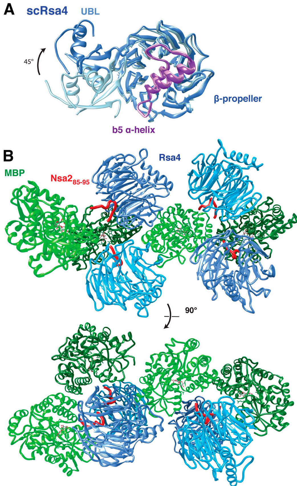
Figure S2. Crystal structures of scRsa4 and scRsa4–scNsa2 complex shown in ribbon representation. (A) Overlay of two different scRsa4 conformations. The scRsa4 crystals contain two molecules in the asymmetric unit (shown in light and darker blue), which differ in the position of the UBL domain with respect to the \beta -propeller domain, indicating a flexible arrangement in solution. Superposition in the \beta -propeller domain shows a rotation of the UBL domain by \sim 45^\circ . (B) The asymmetric unit of the scRsa4–scNsa2 complex. A carrier-driven crystallization approach with MBP was used for structure determination of the minimal scRsa4–scNsa2 complex. Purified Nsa2 (residues 81–101; red) fused to MBP (green) was incubated with Rsa4 (residues 137–515; blue) and SEC purified for crystallization. Crystal contacts are mainly established between MBP and Rsa4 and not directly between neighboring Rsa4 molecules.
