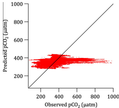
Fig. 1. Multiple linear regression representation of all of the pCO 2 observations in the Chavez et al. (2007) North American Continental Margins dataset. Solid diagonal line represents the perfect-agreement 1:1 relationship.
