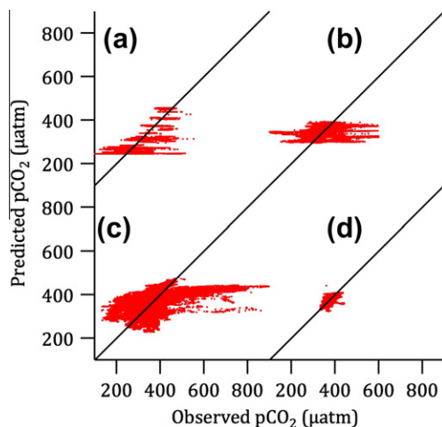
Fig. 2. Comparison of multiple linear regression prediction of sea-surface pCO 2 in the four major coastal sub-regions of North America: (a) Bering Sea and Arctic coastal waters; (b) the Atlantic coast; (c) the Pacific coast; (d) Gulf of Mexico and Caribbean coastal waters. Solid diagonal lines represent the perfect-agreement 1:1 relationship.
