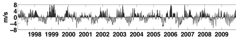
Figure 9. Record of 10 day running averaged daily median N-S wind component ( \text{m s}^{-1} ) from Newport, Oregon, from January 1997 through December 2009. Dark is northward (downwelling favorable), and light is southward (upwelling favorable).
