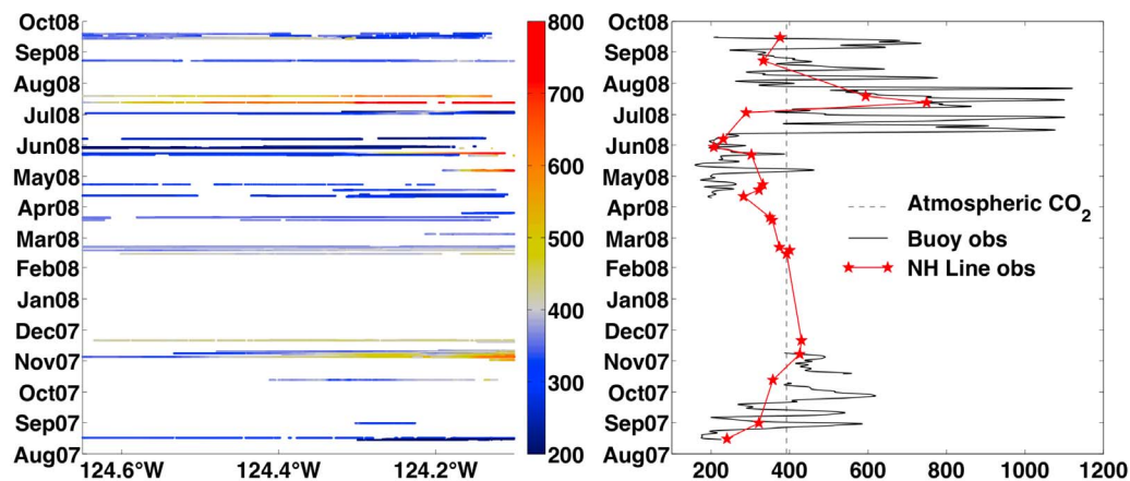
Figure 4. (left) The p\text{CO}_2 ( \mu\text{atm} ) from all cruise data collected over the shelf along the NH line (shown in Figure 1). (right) Buoy and ship (averaged for the central Oregon midshelf region defined in Figure 1) p\text{CO}_2 ( \mu\text{atm} ) data plotted with the average atmospheric p\text{CO}_2 measured during this study (392 \mu\text{atm} ).
