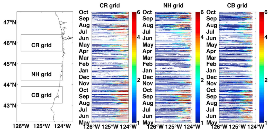
Figure 5. Moderate Resolution Imaging Spectroradiometer (MODIS) Level 2 chlorophyll ( \text{mg m}^{-3} ) from individual satellite passes (usually two per day) from May 2007 to October 2008 for select regions off the Columbia River (CR grid), Newport, Oregon (NH grid), and Coos Bay, Oregon (CB grid). Data are plotted in log scale.
