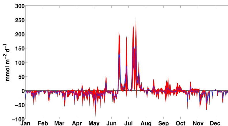
Figure 8. A composite year of sea-air \text{CO}_2 flux ( \text{mmol m}^{-2} \text{d}^{-1} ) on the central Oregon midshelf calculated from NH10 buoy data. The blue line is the daily mean flux, and the red area represents the standard deviation about the daily means.
