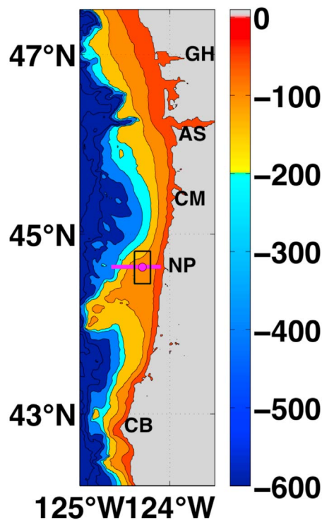
Figure 1. ETOPO1 1–Arc Minute Global Relief Model bathymetry for Oregon highlighting the shelf (0–200 m). Circle near Newport, Oregon, is the position of the NH10 buoy, the platform for our moored system. The east-west bar is the Newport Hydrographic line (NH line) extending from shore out past the shelf break (25 nm). The region where data are selected for construction of a composite year of p\text{CO}_2 (box, dimensions are 44.45°N–44.81°N and 124.3925°W–124.2155°W) is inshore of the 200 m isobath, centered on the NH10 buoy position (44.633°N, 124.304°W), extends ~20 nm in the north-south direction and ~10 nm in the east-west direction, and represents the central Oregon mid-shelf. Bathymetry data are provided by the National Geophysical Data Center ( http://www.ngdc.noaa.gov/mgg/global/global.html ). Coastal locations mentioned in the text are shown: GH, Grays Harbor, Washington; AS, Astoria, Oregon; CM, Cape Meares, Oregon; NP, Newport, Oregon; CB, Cape Blanco, Oregon.
