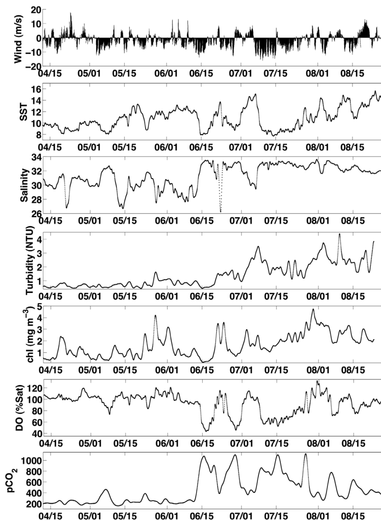
Figure 6. Hourly vector winds ( \text{m s}^{-1} ) from the NOAA C-Man station in Newport, Oregon, and SST ( ^{\circ}\text{C} ), salinity, turbidity (nephelometric turbidity units, NTU), chlorophyll ( \text{mg m}^{-3} ), dissolved oxygen (percent saturation), and p\text{CO}_2 ( \mu\text{atm} ) from the NH10 buoy for the time period 12 April to 28 August 2008.
