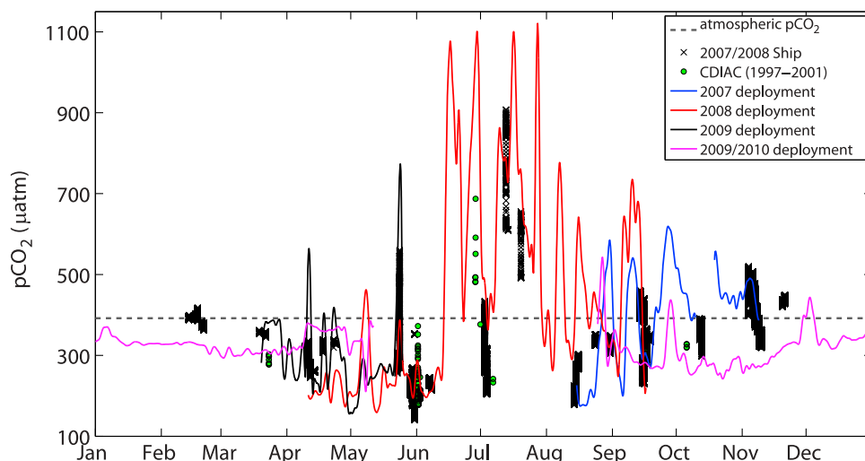
Figure 2. Composite seasonal cycle of p\text{CO}_2 ( \mu\text{atm} ) collected from ships (within the box region defined in Figure 1) and moorings near the NH10 station position off Newport, Oregon.
