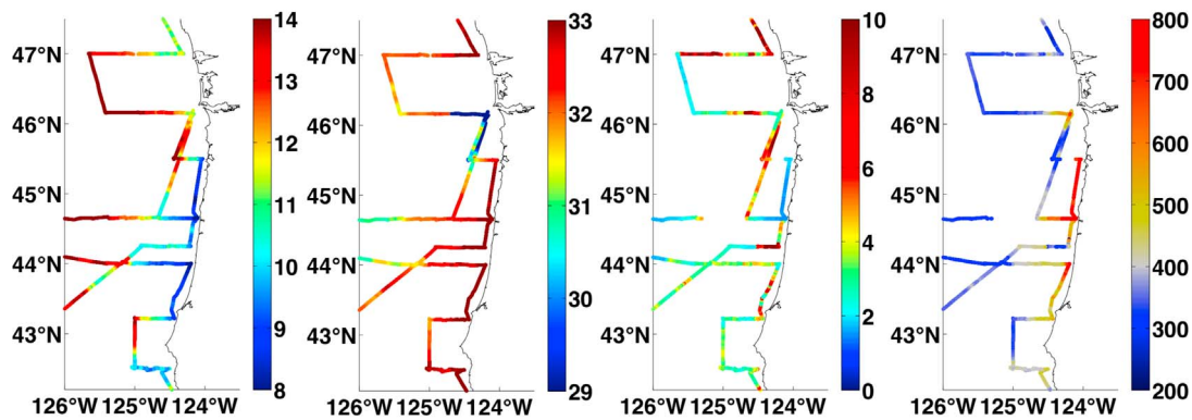
Figure 7. Underway SST ( ^{\circ}\text{C} ), salinity, chlorophyll ( \text{mg m}^{-3} ), and p\text{CO}_2 ( \mu\text{atm} ) from cruises during July 2008.
