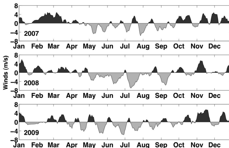
Figure 3. The 10 day running averaged daily median N-S wind magnitude for (top) 2007, (middle) 2008, and (lower) 2009, observed at the NOAA C-Man station in Newport, Oregon. Dark is northward (downwelling favorable), and light is southward (upwelling favorable).
