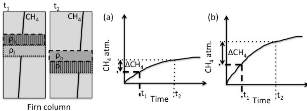
Figure 1. Schematic to illustrate how the layered bubble trapping mechanism can generate high-frequency CH 4 artifacts in ice cores. At time t_1 , air bubbles within the relatively high-density ( \rho_h ) layer are closed off at a relatively shallow depth in the firn column. At time t_2 , air bubbles with the relatively low-density ( \rho_l ) layer are closed off deeper in the firn column. Between t_1 and t_2 the atmospheric concentration of CH 4 is increasing and so the CH 4 concentration in the diffusive column also increases, generating a CH 4 concentration difference \Delta\text{CH}_4 between the bubbles in depth-adjacent layers trapped at t_1 and t_2 . Increasing the atmospheric CH 4 growth rate (b compared to a) results in a larger \Delta\text{CH}_4 . A negative atmospheric growth rate would cause a change in the sign of \Delta\text{CH}_4 .
