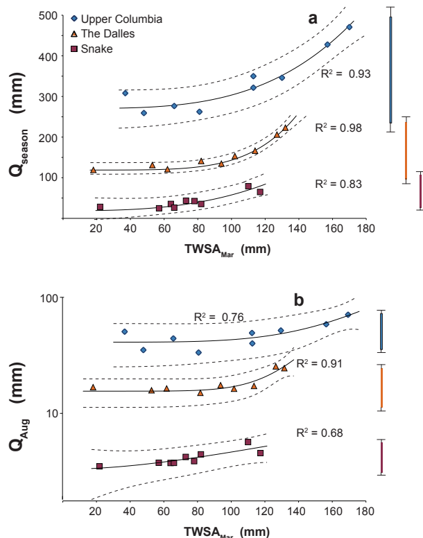
Figure 6. Measurements of terrestrial water storage anomalies in March ( \text{TWSA}_{\text{March}} ) effectively predict the cumulative runoff for April–September ( Q_{\text{season}} ; a ), and describe how these three regional watersheds function as simple non-linear systems. \text{TWSA}_{\text{March}} also predicts mean runoff for August ( Q_{\text{August}} ; b ), one of the driest months of the year when demand for water is at its peak. The hashed lines represent the 95 % confidence intervals. The box plots to the right of each plot represent the range of Q for the respective watershed from WY’s 1969–2012. Note the semi-log y axis on ( b ).
