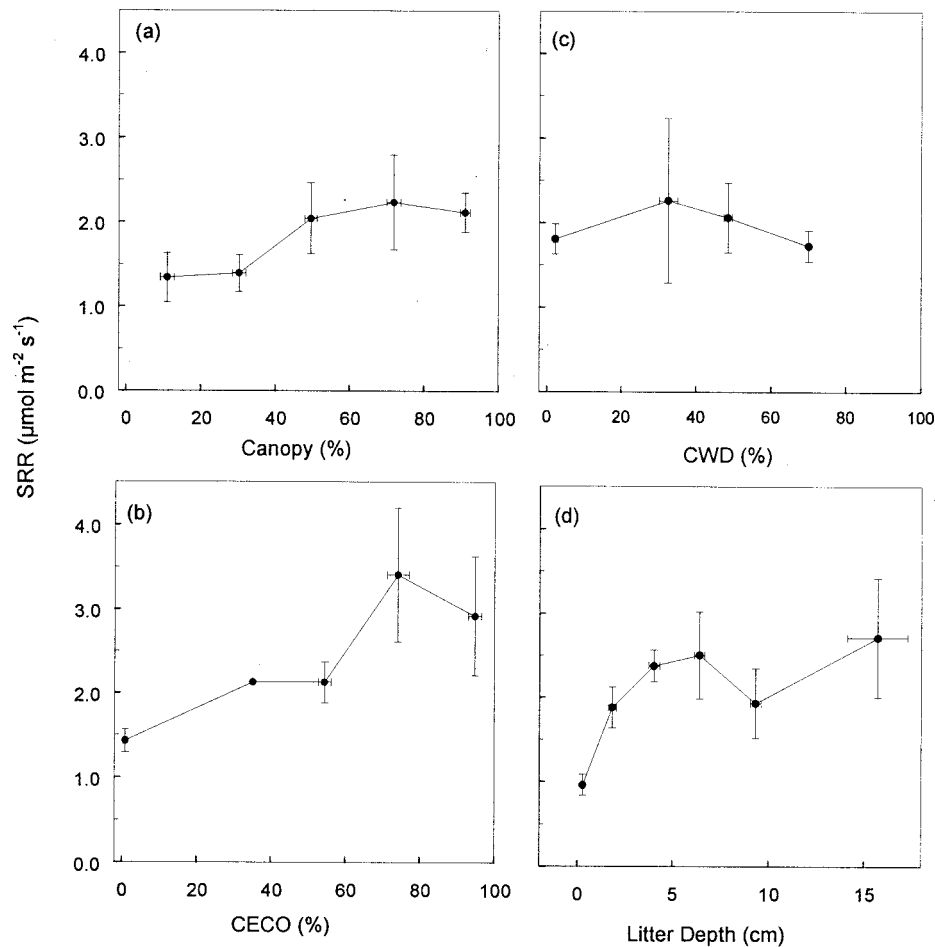
Figure 2. Change in soil respiration rate (SRR) with change in canopy cover, ceanothus shrub cover (CECO), coarse woody debris cover (CWD), and litter depth. Black dots are mean values, and the error bars indicate standard errors.
