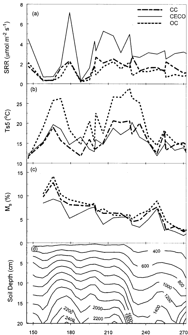
Figure 4. Seasonal changes in (a) soil respiration rate (SRR), (b) soil temperature at 5-cm depth ( T_{s5} ), (c) soil moisture ( M_s ), and (d) CO 2 concentration (ppm) within 0–20 soil depth in three dominant patch types: close canopy (CC), ceanothus shrub (CECO), and open canopy (OC) during May–Oct., 2000.
