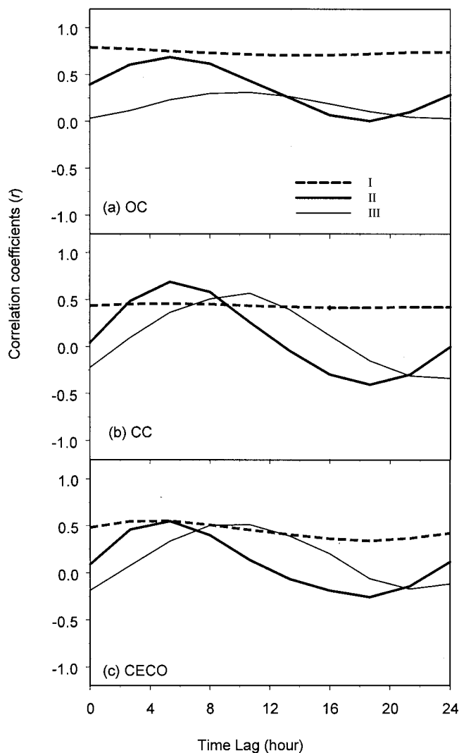
Figure 6. Correlation coefficients ( r ) between soil respiration rate and soil temperature at 5-cm depth ( T_{ss} ) with each 2.5-hour lag time in three patch types: (a) open canopy (OC), (b) closed canopy (CC), and (c) ceanothus shrub (CECSO) at three soil moisture ( M_s ) conditions: I: M_s > 10\% ; II: 5\% < M_s \leq 10\% ; and III: M_s \leq 5\% .
