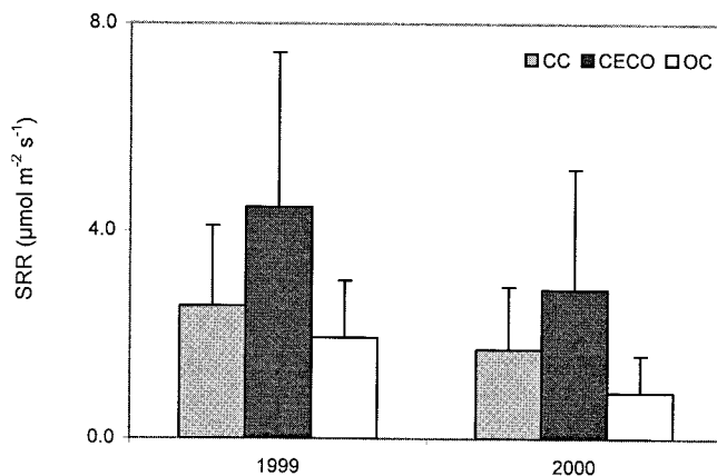
Figure 1. Means and standard deviations of soil respiration rate (SRR) in three dominant patch types of mixed-conifer forest: open canopy (OC), canopy cover (CC), and ceanothus shrub (CECO) during (left) June–Aug. 1999 and (right) May–Oct. 2000.
