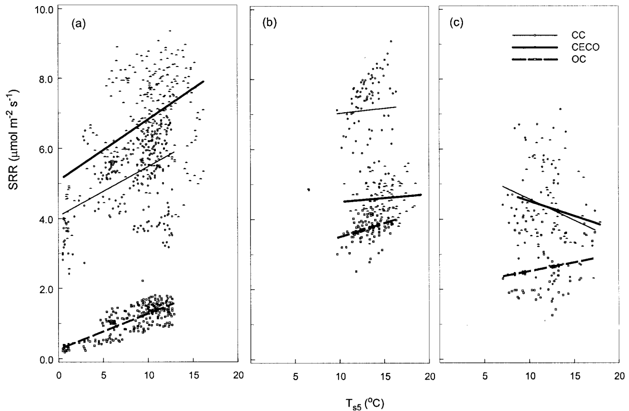
Figure 5. The relationship between soil respiration (SRR) and soil temperature at 5-cm depth ( T_{s5} ) under three soil moisture ( M_s ) conditions: (a) M_s > 10\% , (b) 5\% < M_s = 10\% , and (c) M_s = 5\% in three patch types: canopy cover (CC), ceanothus shrub (CECO), and open canopy (OC). The least-square smoothed lines show the change in the relationships from positive to negative.
