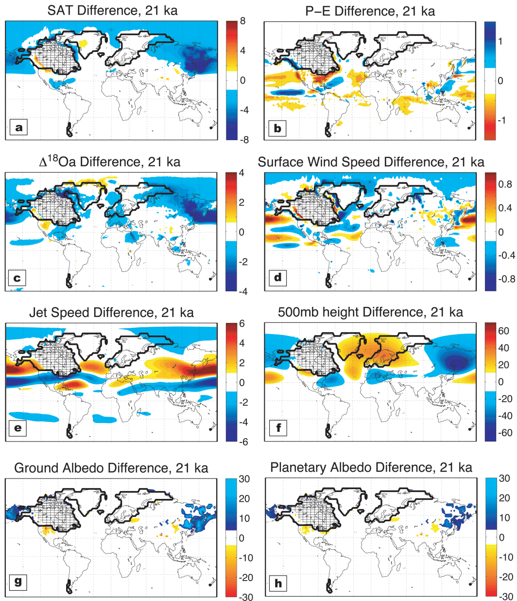
Fig. 2. Differences between 21 ka simulations (21ka-L minus 21ka-5G) for the following annually averaged atmospheric variables: (a) surface air temperature ( ^{\circ}\text{C} ); (b) precipitation minus evaporation ( \text{mm day}^{-1} ); (c) \delta^{18}\text{O}_a (‰); (d) surface wind speed ( \text{m s}^{-1} ); (e) atmospheric jet speed (defined as the wind speed at 250 hPa, \text{m s}^{-1} ); (f) geopotential height at the 500 mb level, with zonal mean removed (m); (g) ground albedo (%); and (h) planetary albedo (%). The LIS is masked out to focus on downstream differences. Ice-sheet extents outlined in bold black lines.
