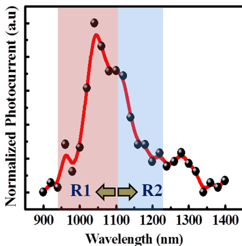
FIG. 7. Normalized photocurrent spectrum of InP QD/Si nano-heterojunction at a reverse bias voltage of -2 V. The individual signature of formation of new band gap at the InP QD/Si interface (R1) and Si band edge (R2) are shown.
