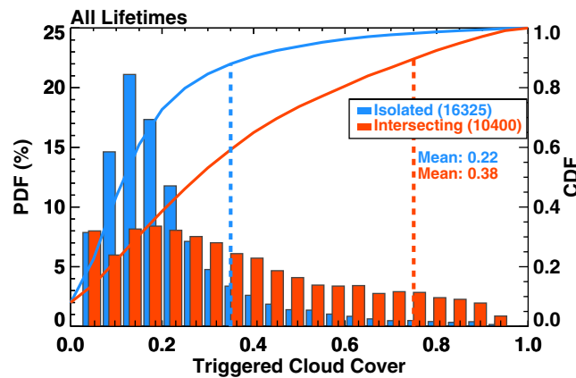
Figure 9. PDF (bars) of triggered cloud cover (cloudy area/cold pool boundary area) for regular (blue) and intersecting (orange) cold pool boundaries, cumulative density function is also plotted in solid lines, with 90th percentile cloud cover value shown in dash lines. The numbers of cold pool sample and mean cloud cover are shown in the legend.
