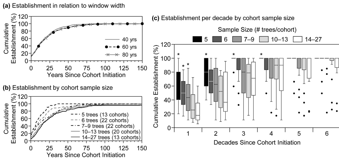
Fig. 3. Comparison of establishment trajectories for Douglas-fir trees in relation to (a) the window width used to estimate the number of cohorts per stand, and (b) the number of trees representing each cohort for cohorts identified using an 80-year window. In (c), cumulative establishment by the end of the first six decades for cohorts identified with the 80-year window is compared across cohorts represented by different numbers of trees. Asterisks indicate a statistically greater percentage of trees established ( p < 0.05 ) than in the group of the largest sample size (14–27 trees) based on a one-tailed Dunn's test conducted after a Kruskal-Wallis test.
