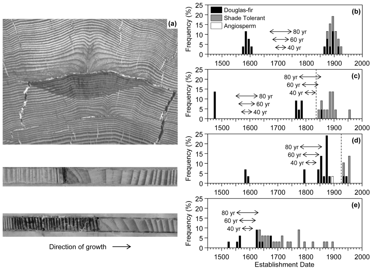
Fig. 2. Illustration of (a) healed fire scars in a Douglas-fir stump (photo by Peter Weisberg) and increment cores. In (b–e), age-structure data for four representative transects illustrate how windows of 40, 60, and 80 years with no record of establishment were used to estimate the number of cohorts per stand. Example (b) is the most common scenario, where two cohorts are identified regardless of window width. The youngest cohort in (c) and (d) was identified based on healed fire scars (vertical dashed lines). Examples (d) and (e) illustrate how using a 40-year window can lead to identification of a greater number of cohorts than 60- or 80-year windows.
