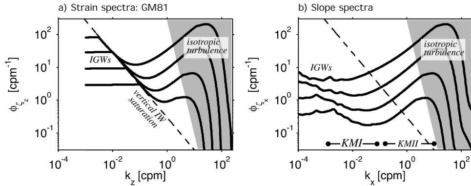
FIG. 1. (a) GM81 strain spectra with saturated internal wave subrange and turbulence for four different energy levels and their corresponding turbulence levels assuming \varepsilon \sim E^2 . After D’Asaro and Lien (2000) except turbulence is added to the internal wave spectrum rather than intersecting them with a sharp change of slope. (b) Slope spectra in the same wave and turbulence fields as calculated in the text (section 6). The same dashed line as in (a) is shown for reference. (The slightly jagged nature of these spectra is due to representing the vertical spectra as discrete modes rather than continuous wavenumbers.) This paper is concerned with the low-wavenumber portion of the horizontal spectra.
