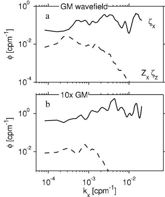
FIG. A1. Comparison of simulated internal wave displacement spectrum and the signal induced by the instrument moving with a path given by \partial Z/\partial x , through the simulated strain field \zeta_x : (a) for a GM wave field and (b) for a GM-shaped wave field with 10 times the energy.
