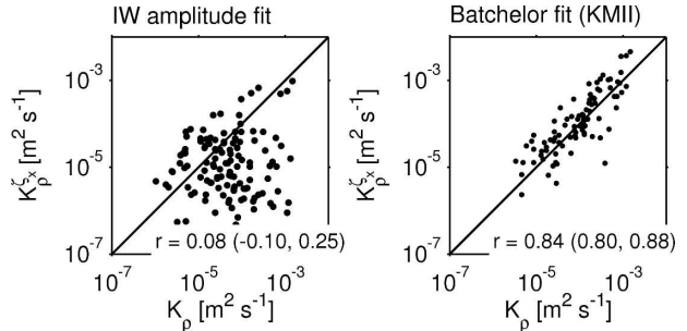
FIG. 12. (a) Comparing the turbulence estimate based on the amplitude of the low-wavenumber slope spectra with the shear probe estimate: the correlation coefficient between these two estimates is shown. (b) Five-kilometer averages of the dissipation estimates made from fitting the high-wavenumber subrange to the Batchelor spectra (described in Part II).
