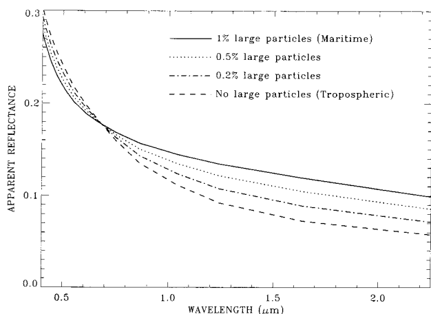
Fig. 4. Examples of simulated reflectances ( \rho_{\text{atm}+\text{sfc}}^* ) as a function of wavelength for four types of aerosol model at the same relative humidity of 50%. The simulations are made for a solar zenith angle of 36^\circ , a view zenith angle of 54^\circ , a relative azimuth angle of 156^\circ , an aerosol optical depth of 0.7 at 0.55\text{ }\mu\text{m} , and a surface wind speed of 6 m/s.
