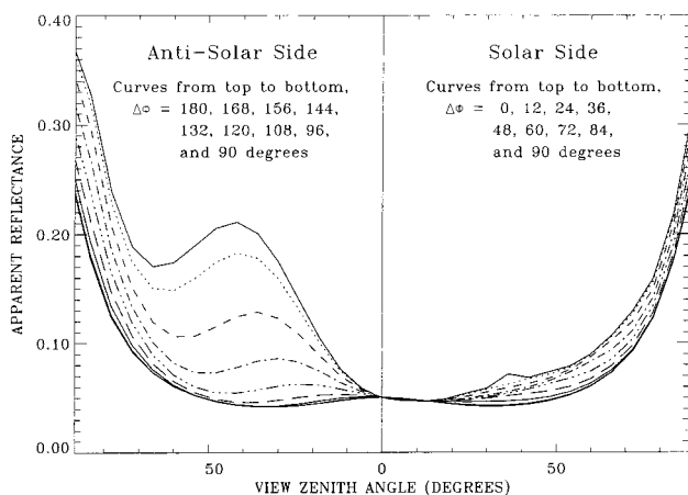
Fig. 3. Examples of simulated 0.61\text{-}\mu\text{m} channel reflectance ( \rho_{\text{atm}+\text{sfc}}^* ) as a function of view angle for several relative azimuth angles. The simulations are made for a solar zenith angle of 36^\circ , an aerosol optical depth of 0.2 at 0.55\text{ }\mu\text{m} , the maritime aerosol model with a relative humidity of 80%, and a surface wind speed of 6 m/s.
