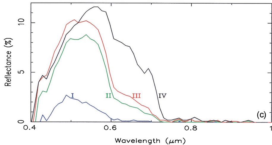
Fig. 9. (a) Color composite image of the AVIRIS scene over the Florida Keys, (b) the radiance spectra extracted from the four areas marked I-IV in (a), (c) the retrieved water-leaving reflectance spectra from the four spectra in (b). During the processing of the color image in (a), the 0.70- \mu\text{m} AVIRIS channel is assigned as the red channel, the 0.55- \mu\text{m} channel as the green channel, and the 0.44- \mu\text{m} channel as the blue channel. The color image is obtained by superposition of the red, green, and blue channel images.
