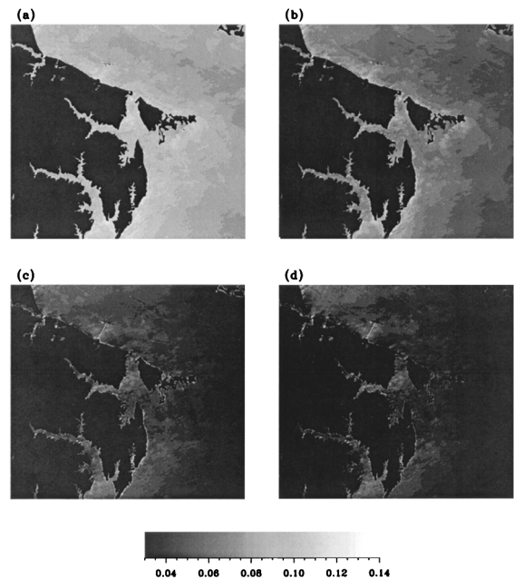
Fig. 7. AVIRIS images of (a) 0.55 \mu\text{m} , (b) 0.66 \mu\text{m} , (c) 0.865 , and (d) 1.04 \mu\text{m} acquired over the mouth of the Chesapeake Bay ( 37^\circ 12' \text{N} and 76^\circ 24' \text{W} ) in eastern Virginia on 17 August 1997.
