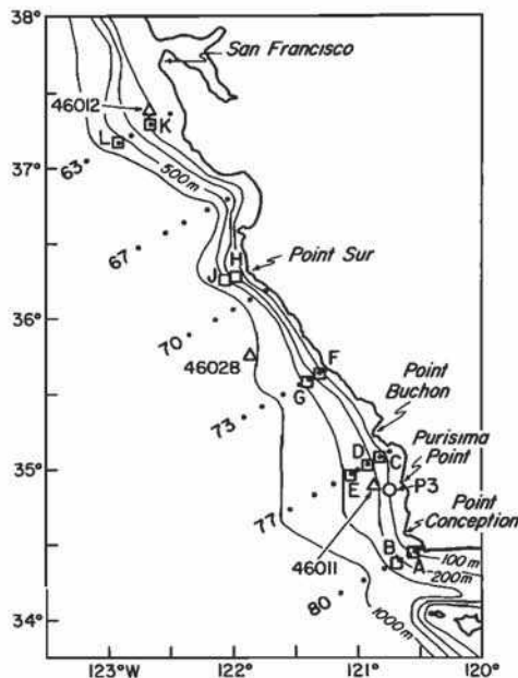
Fig. 2. Map of the central California coastal region. NDBC wind buoys are shown by triangles, CCCCS current meter moorings (labeled A through L, excluding I) are shown by squares, and the SuperCODE mooring P3 is shown as a circle. The dots indicate the locations of the large-scale array of CCCCS conductivity-temperature-depth (CTD) stations with line number labels corresponding to the standard CalCOFI line numbering convention.
