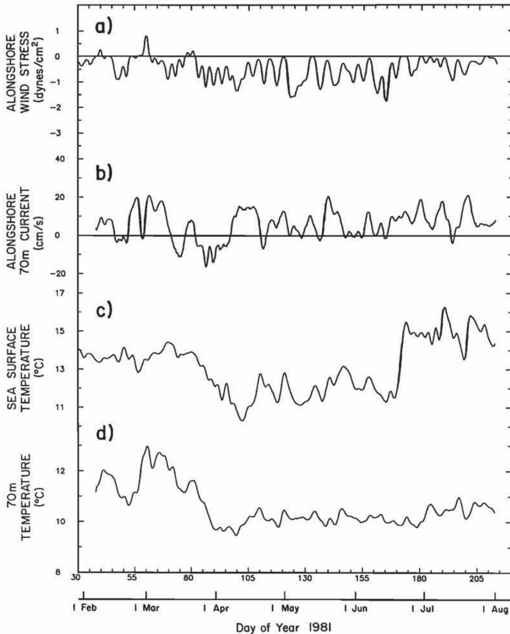
Fig. 8. Time series measurements for the period February through July 1981 of (a) alongshore wind stress at buoy 46011, (b) alongshore currents at 70 m at SuperCODE location P3, (c) sea surface temperature at buoy 46011, and (d) 70-m temperature at location P3. The alongshore direction for winds and currents is defined to be the principal axes determined from the 6 months of data, with positive values poleward ( 323.2^\circ\text{T} for wind stress and 355.9^\circ\text{T} for currents).
