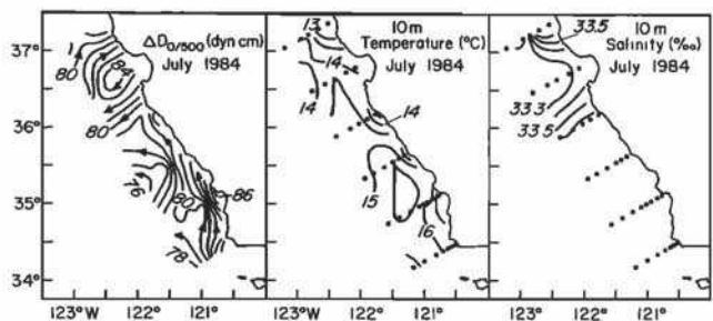
Fig. 14. Maps of (left) the dynamic height of the sea surface relative to 500 dbar, (middle) temperature at 10-m depth, and (right) salinity at 10-m depth from CCCCS CTD measurements during July 1984. Measurements were made between July 4 and 14, 1984.
