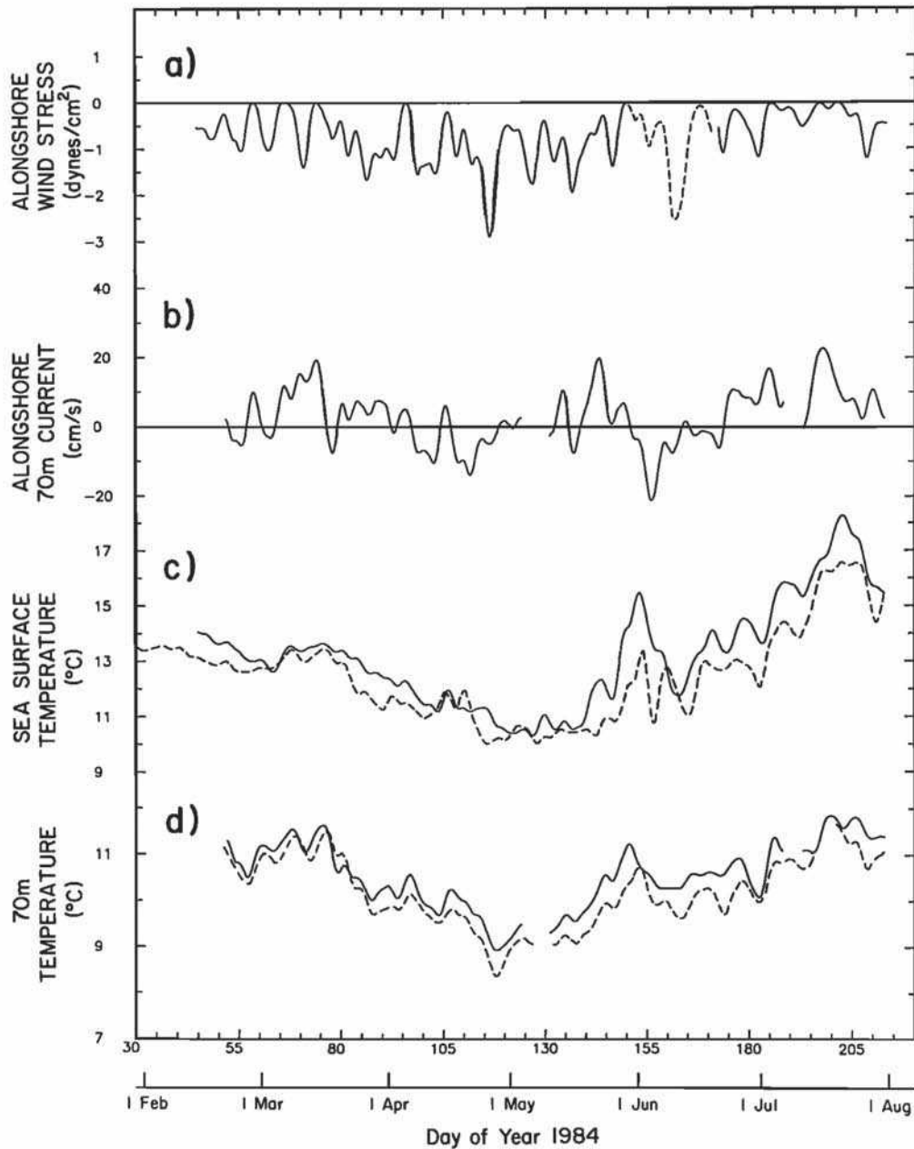
Fig. 4. Time series measurements for the period February through July 1984 of (a) alongshore wind stress at buoy 46011 (the dashed line in the data gap during the first half of June is the wind stress at buoy 46028, 119.5 km to the north); (b) alongshore currents at 70 m at CCCCS site C, (c) sea surface temperature (SST) at buoy 46011, and (d) 70-m temperature at site C. The alongshore direction for winds and currents is defined to be the principal axes determined from the 6 months of data (Tables 1 and 3), with positive values poleward. Dashed lines in Figures 4c and 4d are SST at buoy 46028 and 70-m temperature at CCCCS site F, respectively.
