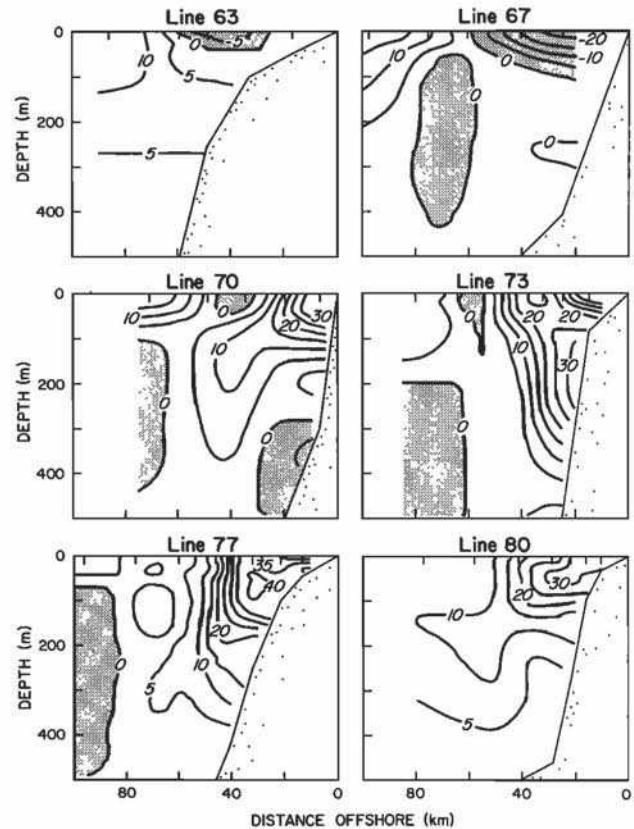
Fig. 17. Vertical sections of July 1984 alongshore geostrophic velocity relative to 500 dbar (contour interval is 5 cm/s) computed from CCCC dynamic height measurements along the six standard CalCOFI lines shown in Figure 2. Tick marks along top of each plot indicate locations of CTD stations. Shaded regions indicate equatorward flow. Dynamic heights used to compute the relative velocities inshore of the 500-m isobath were extrapolated from deeper water using the method described by Reid and Mantyla [1976]. Measurements were made between July 4 and 14, 1984.
