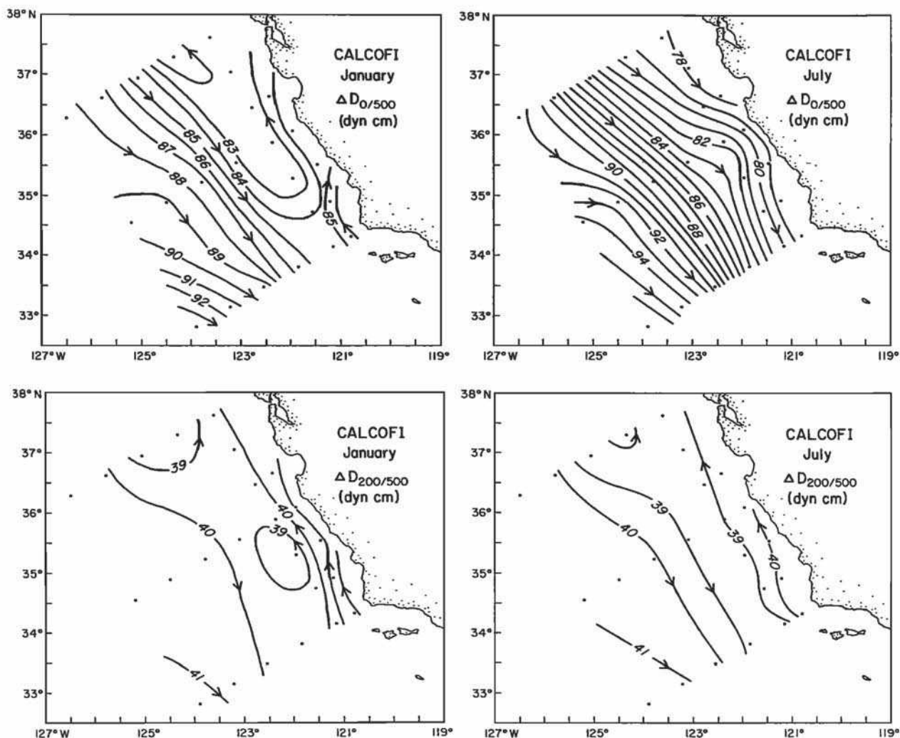
Fig. 1. Seasonal average January and July dynamic heights of the sea surface and 200 dbar relative to 500 dbar off the central California coast. Seasonal averages were determined by harmonic analysis of CalCOFI hydrographic data as described by Chelton [1984].
