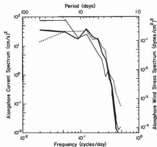
Fig. 7. Variance-preserving spectra of alongshore currents at shelf mooring F (heavy solid line) and upper slope mooring G (thin solid line), and alongshore wind stress at buoy 46028 (dotted line).
