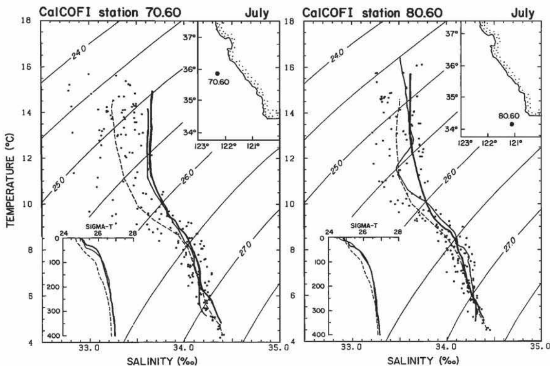
Fig. 10. Temperature-salinity ( T - S ) plots from CalCOFI hydrographic measurements at stations 70.60 and 80.60 over the upper continental slope (see map insets for station locations). The dots correspond to T - S pairs at 16 standard depths from the sea surface to 1000 m for all CalCOFI July measurements between 1950 and 1978. The dashed line through the center of the cluster of dots represents the July seasonal average at the 16 standard depths. The thin and heavy solid lines are the T - S plots from CalCOFI measurements in July 1981 and 1984, respectively. Depths of T - S pairs can be determined from the \sigma_t contours overlaid on the plot and the \sigma_t profiles in the lower left corner of the figure.
