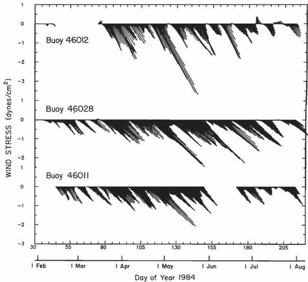
Fig. 3. Stick plot of vector wind stress measured over the period February–July 1984 at the three NDBC buoys shown in Figure 2. Sticks point toward the direction the wind was blowing, and the length of the sticks indicates the magnitude of the wind stress (scale on left axis).
