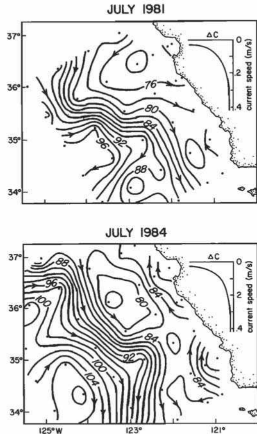
Fig. 9. Dynamic heights of the sea surface relative to 500 dbar determined from CalCOFI hydrographic data for July 1981 and July 1984. Arrows indicate the direction of relative geostrophic flow, and the scale in the upper right corner of each plot indicates the current speed for a given contour separation \Delta C . The data shown in the figures were collected between June 28 and July 5, 1981, and between July 17 and 29, 1984.
