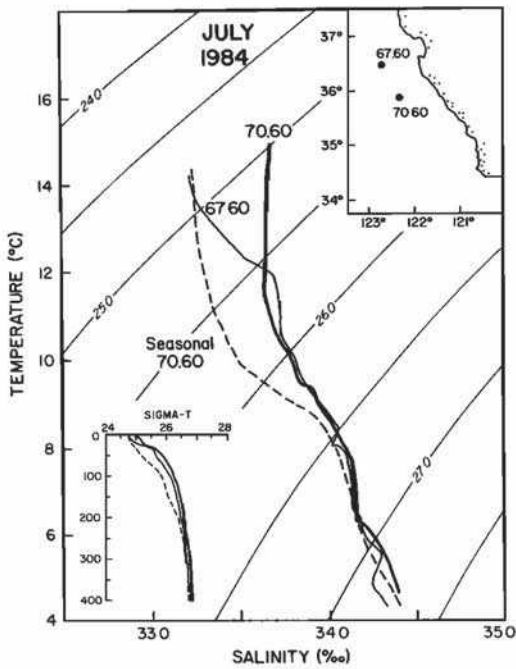
Fig. 15. T - S plots from July 1984 CCCC CTD measurements at standard CalCOFI station locations 67.60 (thin solid line) and 70.60 (heavy solid line). Station locations are shown in the map inset. The dashed line corresponds to the July seasonal average at station 70.60 (from Figure 10). Depths of T - S pairs can be determined from the \sigma_t contours overlaid on the plot and the \sigma_t profiles in the lower left corner of the figure.
