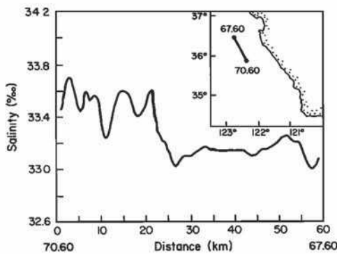
Fig. 16. Salinity measured by the shipboard underway thermosalinograph along the transect from station 70.60 to station 67.60 shown in the map inset. The locations of the two stations are labeled along the distance axis on the bottom.
