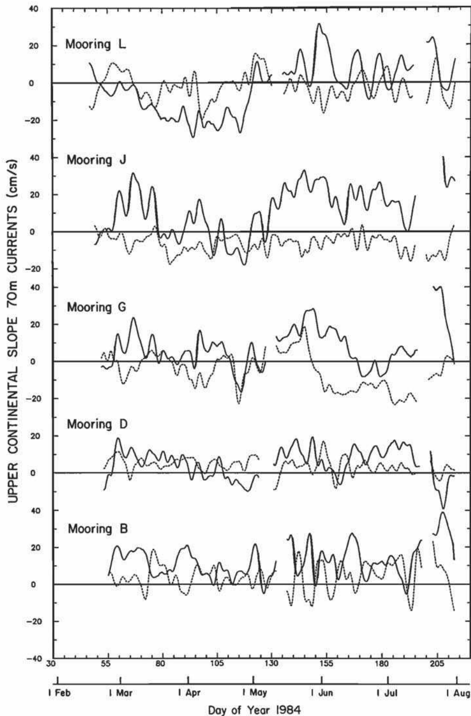
Fig. 6. Alongshore (solid lines, positive poleward) and cross-shore (dashed lines, positive onshore) currents at 70 m over the upper continental slope at CCCCS moorings B, D, G, J, and L for the period February–July 1984. Alongshore and cross-shore directions at each site were defined by the principal axes determined from the 6 months of data (Table 3).
