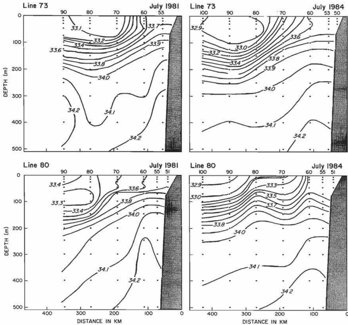
Fig. 12. Vertical sections of salinity from CalCOFI measurements along lines 73 and 80 during July 1981 and 1984.
