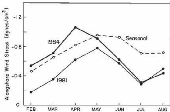
Fig. 13. Monthly average alongshore wind stress at buoy 46011 during 1984 (heavy solid line) and 1981 (thin solid line), and the seasonal average at 35°N (dashed line) determined from 100 years of ship observations [from Nelson, 1977]. Note that the y axis is inverted.
