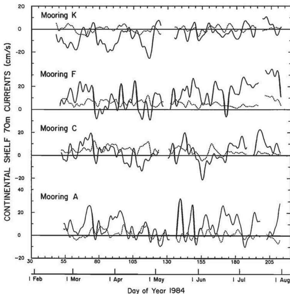
Fig. 5. Alongshore (solid lines, positive poleward) and cross-shore (dashed lines, positive onshore) currents at 70 m over the continental shelf at CCCCS moorings A, C, F, and K (the mooring at site H was lost) for the period February–July 1984. Alongshore and cross-shore directions at each site were defined by the principal axes determined from the 6 months of data (Table 3).
