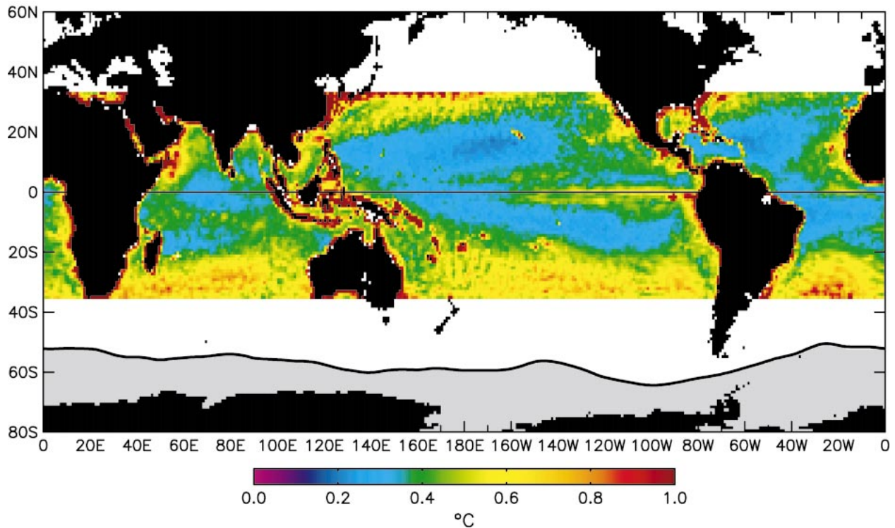
FIG. 1. A global map of the root-mean-square (rms) difference between the weekly averaged TMI SST and the weekly averaged Reynolds SST analyses. Also shown is the northernmost extent of the Antarctic sea ice over the analysis region for the period 1 Aug 1999–31 Jul 2001. The area masked from the analysis is shaded in gray.
