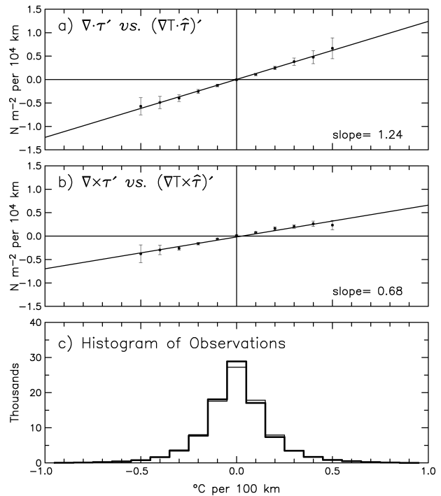
FIG. 7. Binned scatterplots of the relationships between the spatially high-pass-filtered SST and wind stress fields: (a) the perturbation wind stress divergence, \nabla \cdot \hat{\tau}' , plotted as a function of the perturbation downwind SST gradient, (\nabla T \cdot \hat{\tau})' ; (b) the perturbation wind stress curl, \nabla \times \hat{\tau}' \cdot \mathbf{k} , plotted as a function of the perturbation crosswind SST gradient, (\nabla T \times \hat{\tau})' \cdot \mathbf{k} ; and (c) histograms of the number of observations within each bin for (a) (thick line) and (b) (thin line). The points in (a) and (b) are the means within each bin computed from the 11 individual 3-month averages, and the error bars are \pm 1 std dev of the means within each bin. The lines through the points represent least squares fits of the binned overall means to straight lines.
