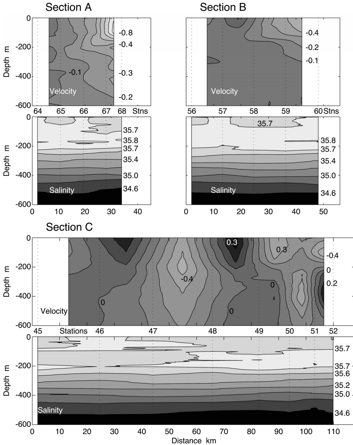
FIG. 3. Cross sections of geostrophic velocity, relative to 1000 decibars, and salinity on Sections A, B, and C derived from the CTD data. Eastward velocity ( \text{m s}^{-1} ) is positive and the contour interval is 0.1 \text{ m s}^{-1} . Salinity contour interval is 0.1 for salinity greater than 35.6 psu and 0.2 for lower salinity.
