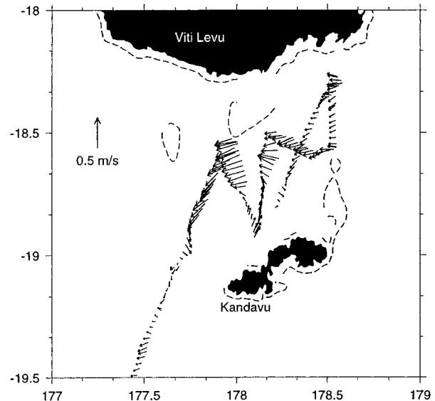
FIG. 2. Current vectors at 110-m depth from the ADCP survey.
