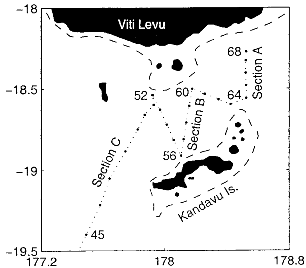
FIG. 1. The survey area south of Fiji showing the ADCP transects and the CTD stations undertaken over the period 11–13 September 1992. Stations 43–52 are the northern end of the WOCE P14C line, while Stations 53–68 were supplementary CTD stations. The 500-m bathymetric contour is shown dashed.
