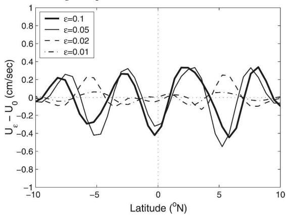
FIG. 12. Similar to Fig. 9: dependence of the 5-yr model mean (years 31–35) depth-averaged (layers 1–7) zonal velocity, U_\varepsilon , along 219°E (141°W) on \varepsilon for the Gent–Cane model forced with symmetric mean plus asymmetric perturbation winds. (top) Zero perturbation depth-averaged zonal velocity, U_0 , (bottom) U_\varepsilon - U_0 given \varepsilon = 0.01 (dash-dot line), 0.02 (dashed line), 0.05 (thin solid line), and 0.10 (thick solid line).
