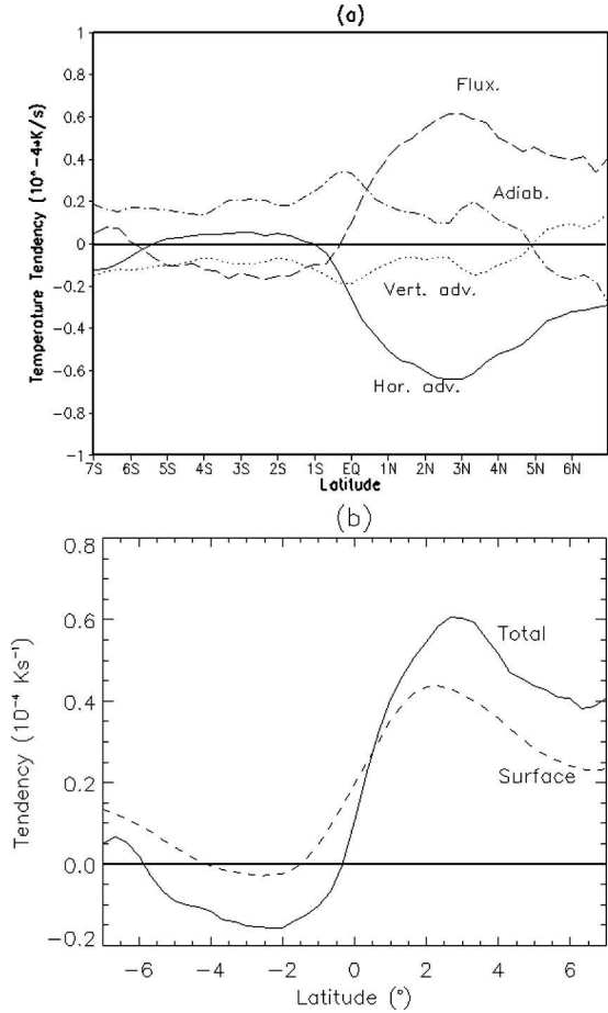
FIG. 9. (a) Vertically averaged temperature budget at 95°W, 2-month mean. All quantities are averaged (mass weighted) to 900 m, with units of 10 -4 K s -1 . “Adiab.” denotes adiabatic warming, “Hor. adv.” denotes horizontal advection, “Vert. adv.” is vertical advection, and “Flux” includes vertical mixing and radiative fluxes terms (see text). (b) Comparison of total flux and the surface heating contribution. The zero line is marked for reference in (a) and (b).
