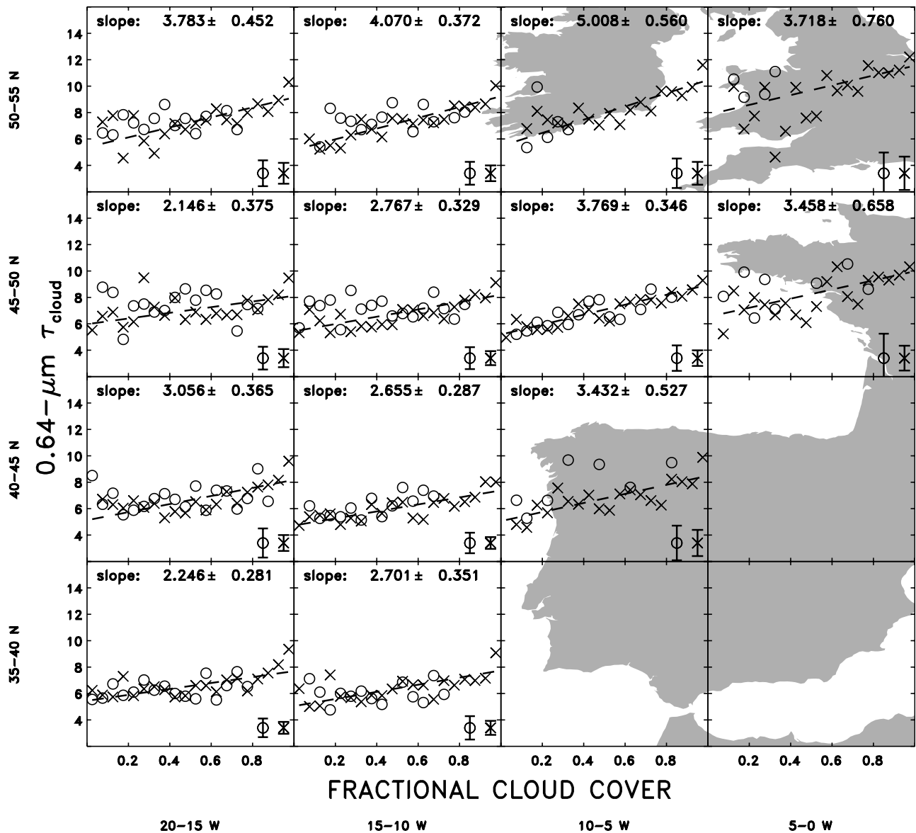
Figure 6. Means of daily averaged 0.64\text{-}\mu\text{m} cloud optical depth for 1^\circ latitude-longitude regions binned for each 0.05 interval of fractional cloud cover. Each subpanel contains data from that 5^\circ \times 5^\circ latitude-longitude region. Circles are data for 1^\circ regions that contained sufficient observations of both aerosol and cloud properties to be included in Figures 3–5. Crosses are data from 1^\circ latitude-longitude regions that passed the screening tests for single-layered, low-level clouds but lacked a sufficient number of aerosol retrievals to be included in the aerosol-cloud associations. The root-mean-square of the standard error (as described in Figure 3) for the two data sets are shown in the bottom right corner of each panel. The dashed line is a linear fit to the bin means of the combined data sets inversely weighted by the standard errors of the combined data sets. Also given are the mean and standard deviation estimated for the slope of the linear fit.
