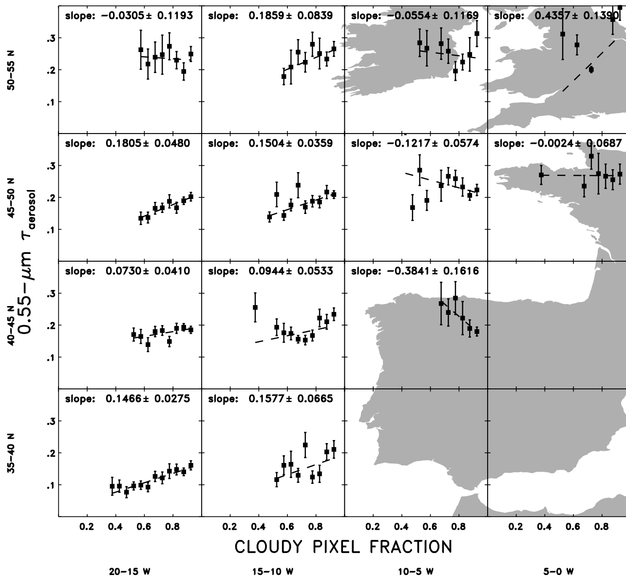
Figure 8. Same as Figure 3 but for 0.55\text{-}\mu\text{m} aerosol optical depth and cloudy pixel fraction. Cloudy pixel fraction is the fraction of pixels within a 1^\circ latitude-longitude region that were identified as containing clouds (pixel-scale cloud fraction, A_c > 0.2 ).
