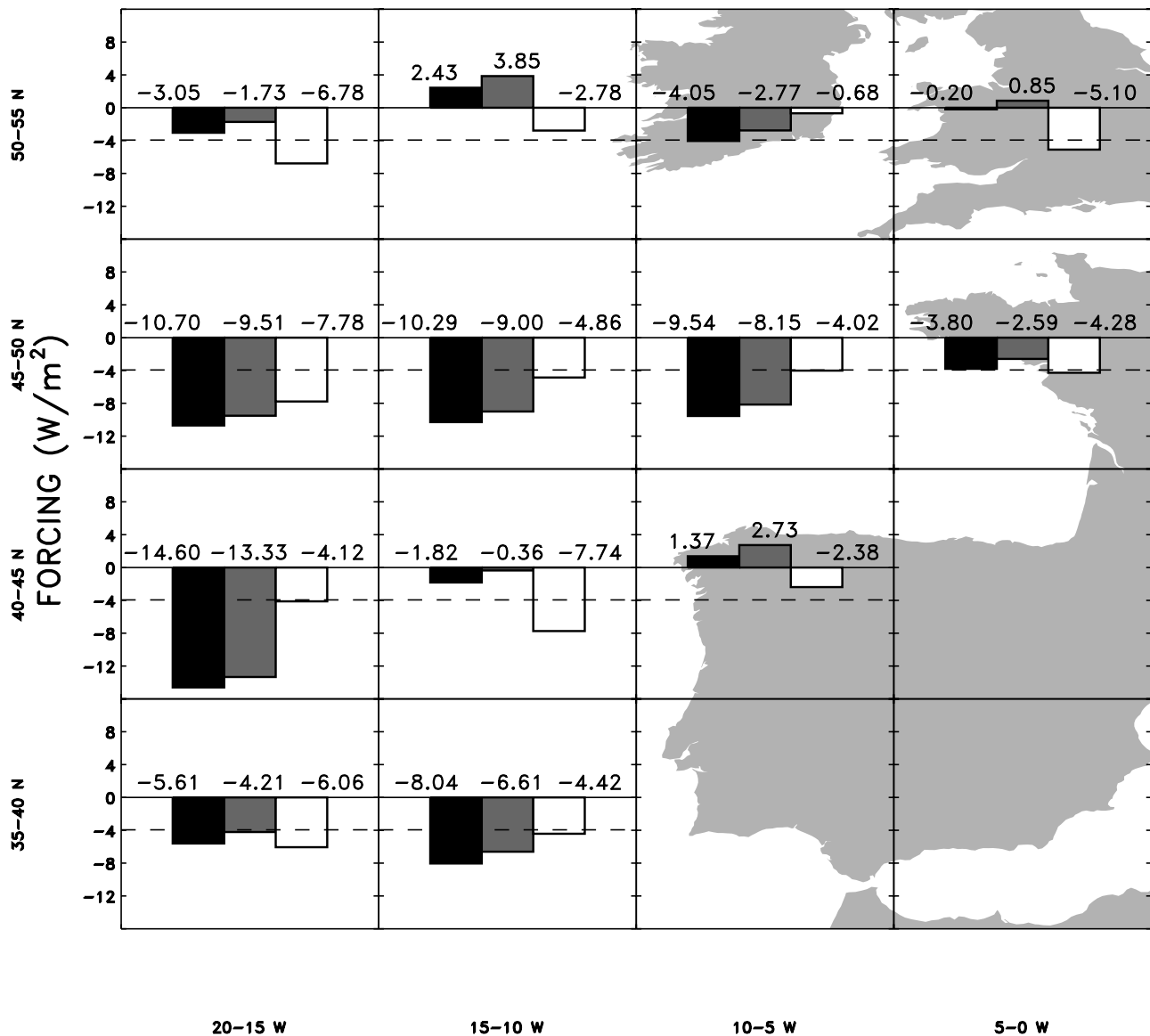
Figure 9. Radiative forcing estimates ( \text{W}/\text{m}^2 ) for an arbitrary increase of 0.55\text{-}\mu\text{m} aerosol optical depth of 0.1 (from 0.15 to 0.25). Solid bars are the forcings for overcast conditions calculated using the changes in cloud optical depth taken from the linear fits in Figure 4 and an increase of the aerosol optical depth below the cloud. Shaded bars are the same forcing as the black bars except the aerosol optical depth was held at the “background” level. Open bars are the forcings for overcast conditions calculated using the changes in droplet effective radius taken from the linear fits in Figure 3 and assuming a constant liquid water path. The dashed line is the aerosol direct radiative forcing for cloud-free conditions ( -3.94 \text{ W}/\text{m}^2 ).
