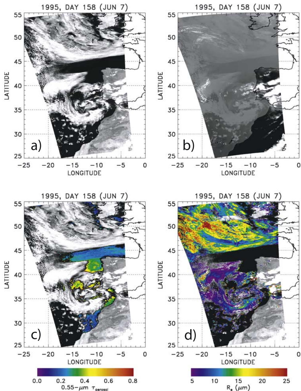
Figure 1. Images of the study region on 7 June 1995, dominated by low-level, single-layered stratocumulus off the west coast of Europe. (a) 0.84- \mu\text{m} 4-km AVHRR reflectances. (b) 11- \mu\text{m} radiances. Upper-level clouds (light objects) overlie a portion of the low-level clouds. (c) Same as Figure 1a but overlain with 0.55- \mu\text{m} aerosol optical depth. (d) Same as Figure 1a but overlain with droplet effective radius ( \mu\text{m} ).
