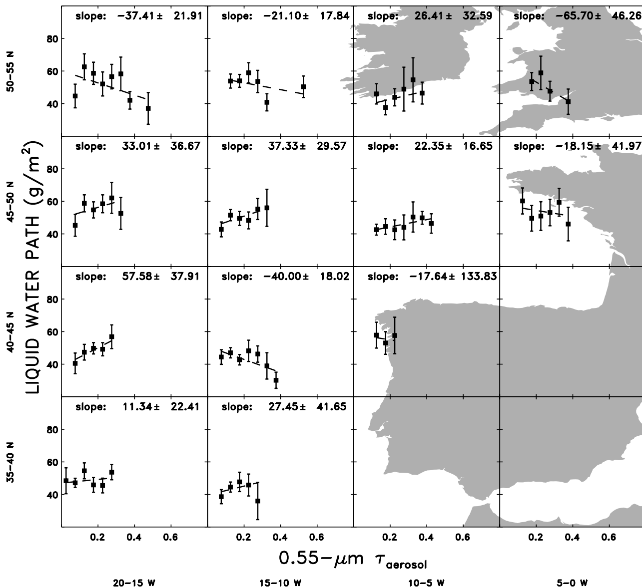
Figure 5. Same as Figure 3 but for cloud liquid water path ( \text{g}/\text{m}^2 ) and 0.55\text{-}\mu\text{m} aerosol optical depth.
