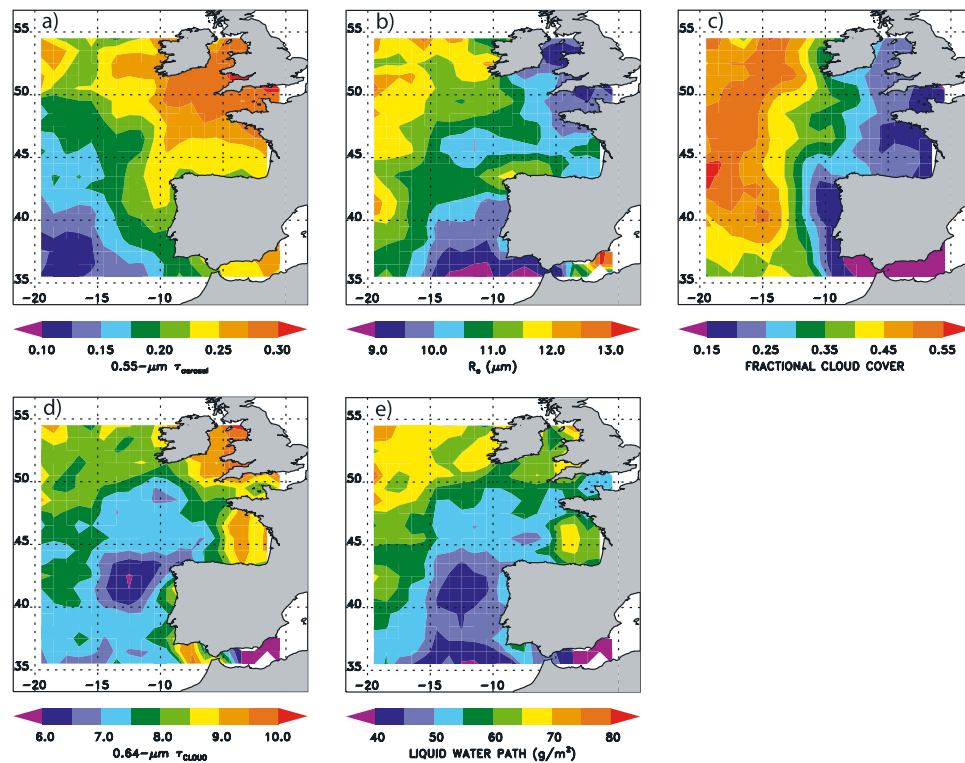
Figure 2. Summertime (May to August 1995) average properties of single-layered, low-level clouds and aerosols. Contour data have been smoothed to show large-scale trends. (a) 0.55- \mu\text{m} aerosol optical depth. Aerosol data from 1^\circ \times 1^\circ latitude-longitude regions that contained clouds that were not part of a single-layered, low-level cloud system were not included in the analysis. (b) Droplet effective radius ( \mu\text{m} ). (c) Fractional cloud cover. (d) 0.64- \mu\text{m} cloud optical depth. (e) Liquid water path ( \text{g}/\text{m}^2 ). In Figures 2b–2e, data were limited to 1^\circ latitude-longitude regions that contained only low-level, single-layered cloud systems. In calculating the pass averages within a region, cloud properties were weighted by the pixel-scale fractional cloud cover.
