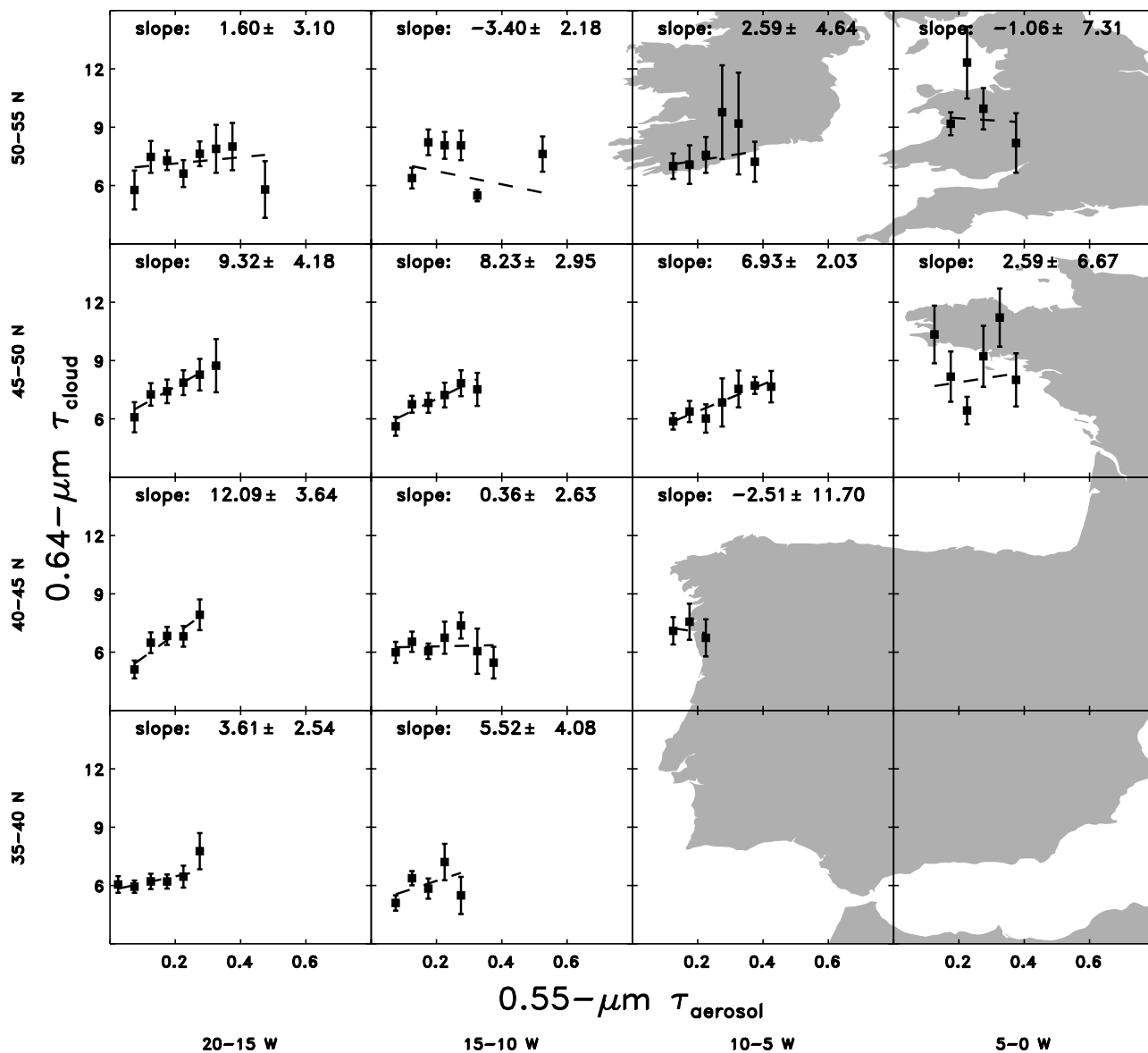
Figure 4. Same as Figure 3 but for 0.64- \mu\text{m} cloud optical depth and 0.55- \mu\text{m} aerosol optical depth.
