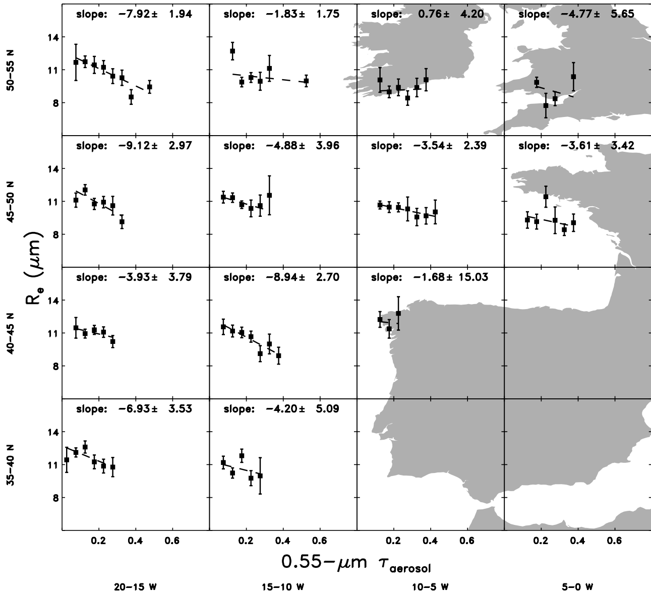
Figure 3. Means of daily averaged droplet effective radius ( \mu\text{m} ) for 1^\circ latitude-longitude regions binned for each 0.05 interval of aerosol optical depth. Each subpanel contains data from that 5^\circ \times 5^\circ latitude-longitude region. Error bars represent the standard error, given by the standard deviation of the means from individual days for that bin divided by the square root of the number of days that contributed observations to that bin. The dashed line is a linear fit to the bin means inversely weighted by the standard errors. Also given are the mean and standard deviation estimated for the slope of the linear fit.
