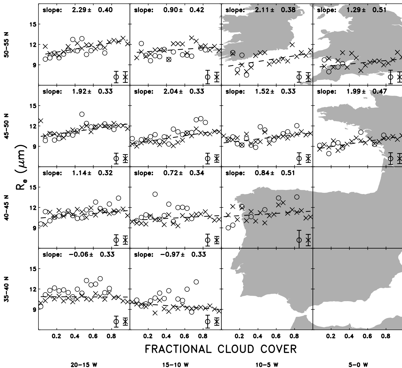
Figure 7. Same as Figure 6 but for droplet effective radius ( \mu\text{m} ) and fractional cloud cover.
