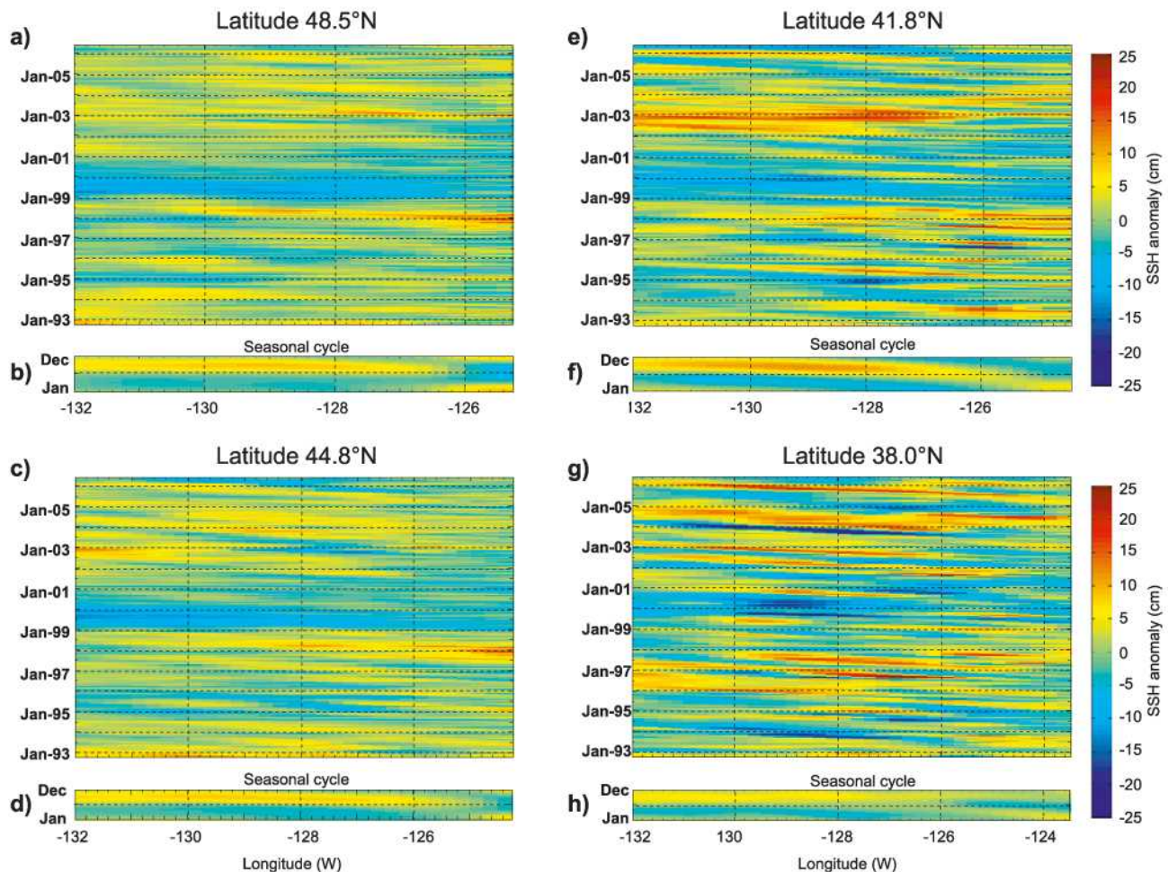
Figure 4. Time-longitude Hovmöller plots of (a) sea level anomaly, with seasonal (annual + semiannual) cycle removed, along latitude 48.5°N, (b) the removed seasonal cycle, (c, d) as above but along 44.8°N, (e, f) along 41.8°N, (g, h) along 38.0°N.
