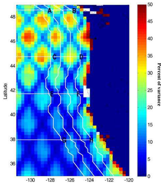
Figure 2. Average error in sea level anomaly due to mapping, expressed as percent of total sea level variance. Estimates at each location were calculated by temporally averaging the error estimates provided by AVISO over the full study period of October 1993 to May 2006. Analysis locations are shown as in Figure 1.
