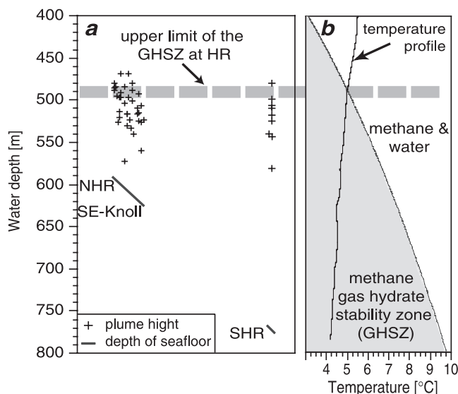
Figure 5. Relationship between the height of the acoustic backscatter images from 12 and 18.5 kHz sources and the upper limit of the gas hydrate stability zone. (a) shows the heights of the acoustic signals at NHR, SEK and SHR (crosses) and the corresponding sea floor depth (bar). In (b) the upper limit of the gas hydrate stability field (gray) at HR is derived from an equation of Dickens and Quinby-Hunt [1994] for pure methane gas using the temperature profiles taken at SHR during the cruise AT3-35b [Torres et al. , 1999].
