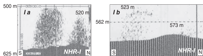
Figure 3. Examples of the variable strength and width of acoustic plumes at NHR from crossings I a and I b (see Figure 2). The depths indicated above the acoustic signals mark the upper limits of the detected backscatter. The x-axis is not in scale.
