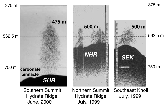
Figure 4. Similar height of the acoustic signals from the vent sites at SHR, NHR and SEK. The depth above the acoustic signals marks their upper limit.
