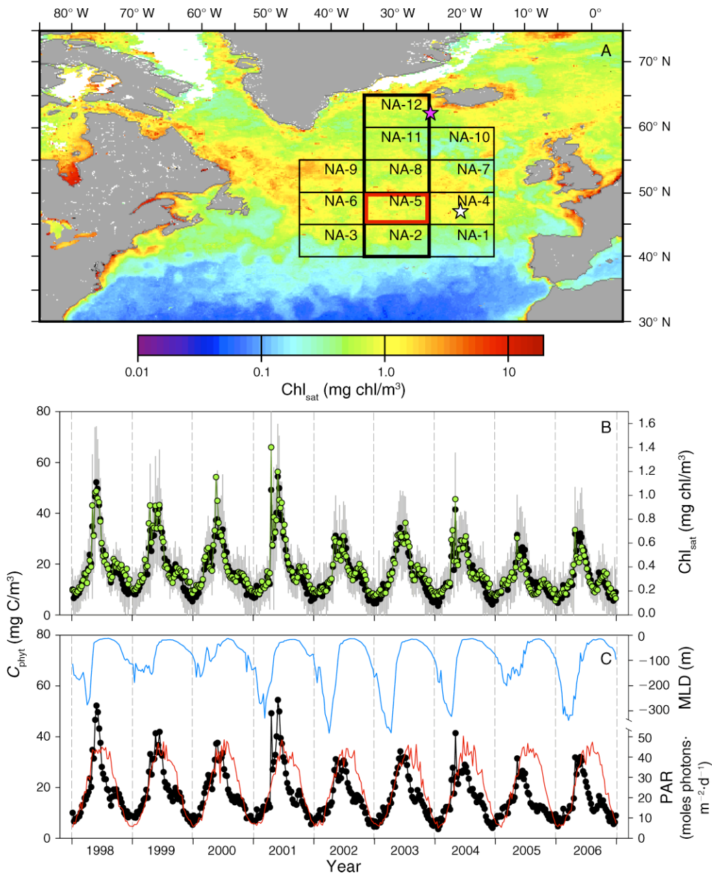
FIG. 1. (A) Typical late bloom surface chlorophyll concentrations ( Chl_{sat} ; note log scale) as observed from the satellite Sea-viewing Wide Field-of-view Sensor (SeaWiFS) in June 2002. Also shown are the 12 study bins and their designations. Red box: Figs. 1B, C, 2A, C, 3, and 4A–C show results from bin NA-5. Heavy black box: bins used in Fig. 2B–F. White star: 1989 North Atlantic Bloom Experiment (NABE) location. Pink star: 2008 North Atlantic Bloom (NAB) study location. (B) Nine-year record of phytoplankton biomass ( C_{phyt} ; black symbols, left axis) and Chl_{sat} (green symbols, right axis) at eight-day resolution for bin NA-5. Gray bars indicate within-bin standard deviations for C_{phyt} . (C) Nine-year record of C_{phyt} (black symbols, left axis, same as panel B), photosynthetically active radiation (PAR; red line, lower right axis), and mixed layer depth (MLD; blue line, upper right axis) for bin NA-5. Vertical dashed lines in panels B and C indicate 1 January of each year.
