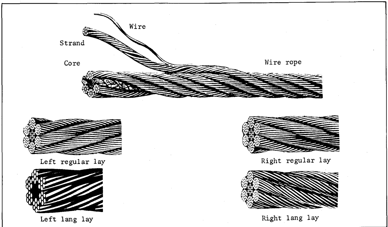
Fig. 2. Composition of wire rope (U.S. Steel Supply, 1975).
