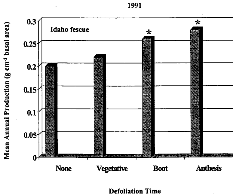
Figure 2. Plant species response to defoliation. Mean relative annual production of Idaho fescue collections from central Oregon grown in a common garden. Values represent the average of all collections: defoliation occurred at vegetative, boot, or anthesis stages of growth. Significant difference in values noted with an *. From Jaindl et al. (1994).
