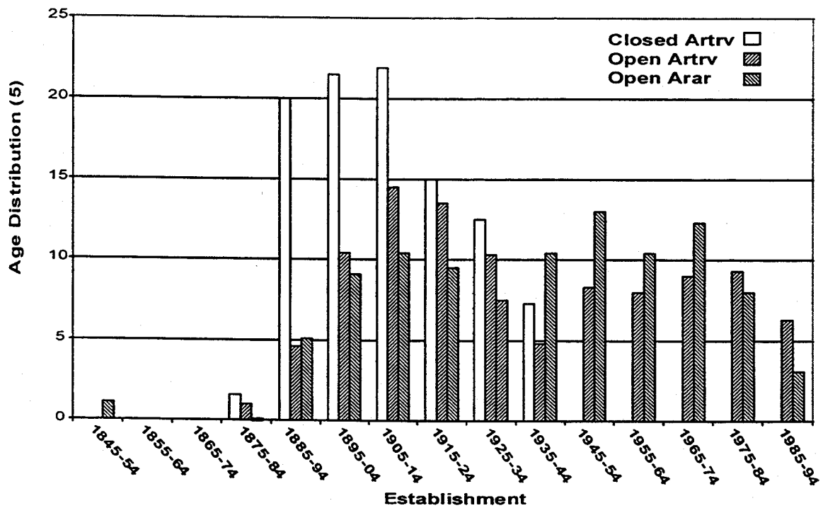
Figure 2. Age distribution (%) of western juniper trees by decade for open low sagebrush (ARAR) (n=88), and open and closed mountain big sagebrush (ARTRV) (n=422).
