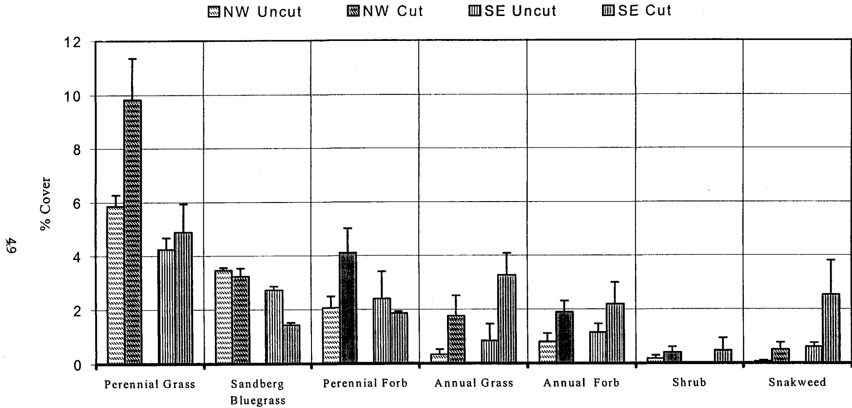
Figure 4. Plant cover by functional groups and species on UNCUT and CUT blocks the third year post treatment.
