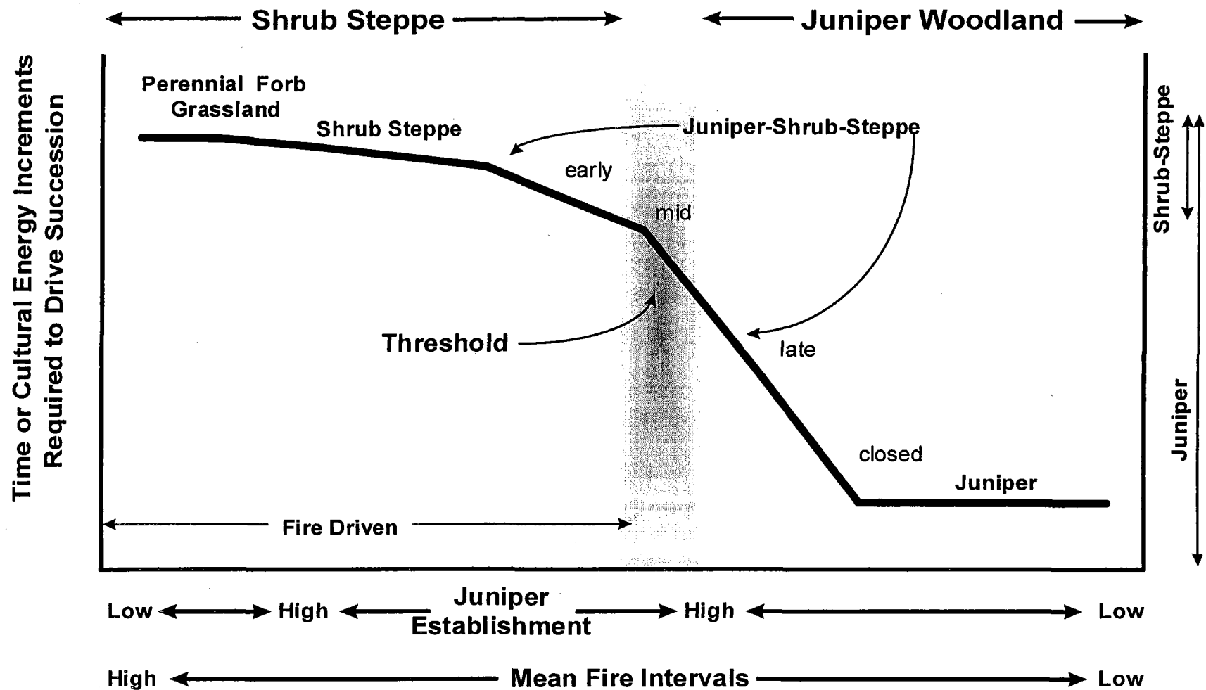
Figure 5. Conceptual diagram of changes in a shrub steppe community in the absence of fire (modeled after Archer 1989). In the absence of fire the abundance of shrubs decline as juniper trees gain dominance. A threshold has been crossed when understory fuels drop to a level where fire is unlikely to carry through the stand or generate enough heat to kill trees > 3m tall. The probability of the woodland crossing the threshold and reverting back to shrub steppe is very low in the absence of a major disturbance or very costly inputs. Tree establishment declines due to a decrease in seed input and safe sites provided by shrubs.
