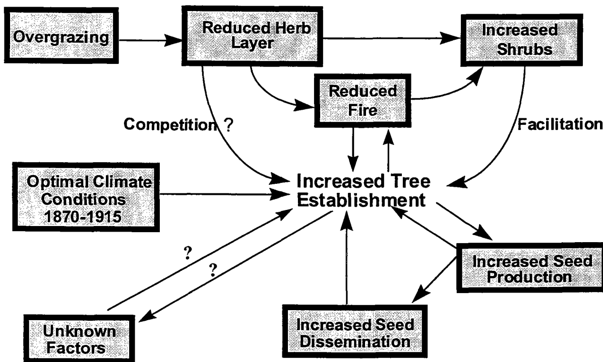
Figure 1. A conceptual model illustrating several key factors that contributed to the expansion of western juniper in the late 1800s and early 1900s. Unknown factors might include increased atmospheric CO 2 , ending of the Little Ice Age, etc.
