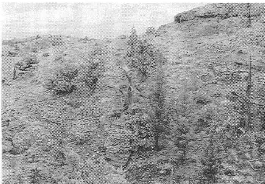
Figure 5. Ancient western juniper trees growing on sedimentary soils in central Oregon.
