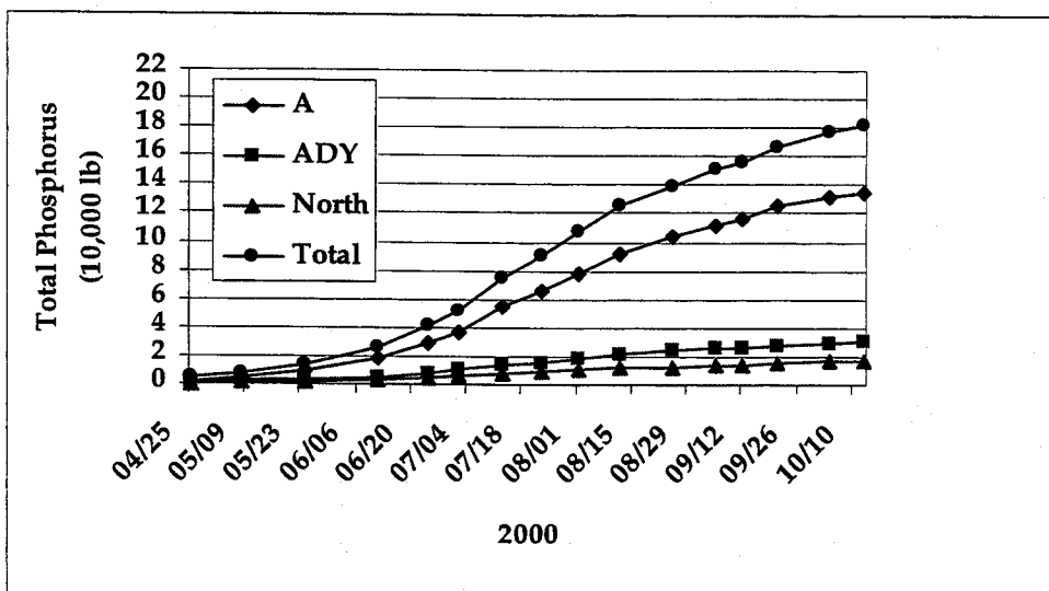
Figure 3. Total phosphorus loading in the Klamath Irrigation Project from the A, North, and ADY canals in 2000.
