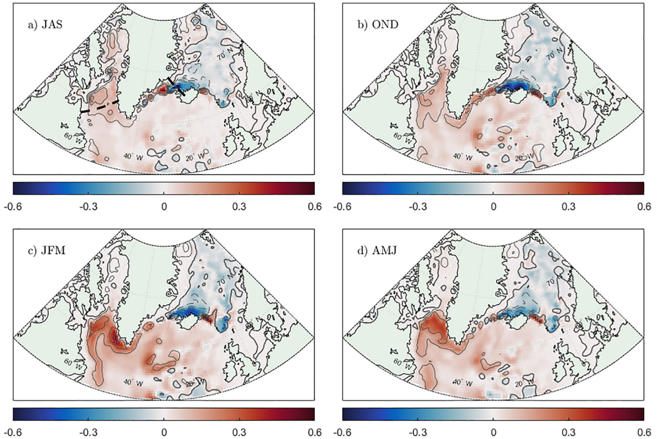
Figure 7. (a–d) Stochastic pressure gradient force Run minus Control Run of indicated 50-year seasonal mean of potential temperature (colormap) and salinity (contour lines in increments of 0.03 psu) at 2.5 m. The dashed black line near Denmark Strait in panel a represents the location of the transect in Figure 6, oriented such that distance increases to the East of Greenland. The dashed black line in the Labrador Sea represents the location of the transect in Figure S9 in Supporting Information S1.
