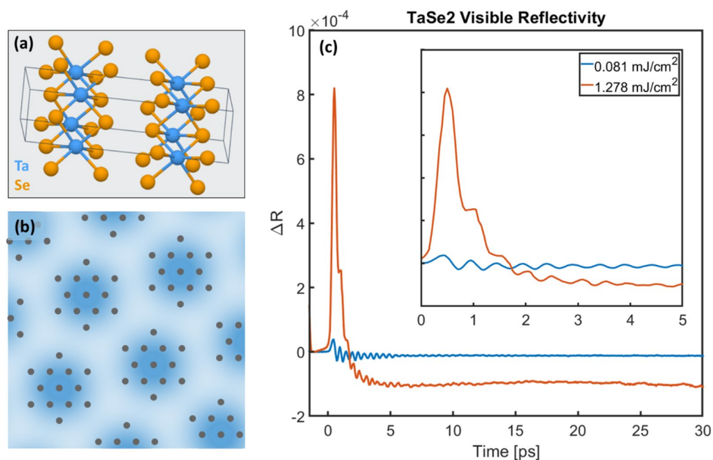
Figure 1. (a) Crystal structure of 1T-TaSe 2 formed by Se-Ta-Se sandwiched layers; blue = Ta, yellow = Se. (b) Cartoon of the 2D CDW in 1T-TaSe 2 ; grey dots represent the Ta atoms (atomic displacements exaggerated) while blue represents electron density (dark blue corresponding to high electron density). (c) Transient reflectivity of TaSe 2 taken with high (orange) and low (blue) pump fluences. Electron excitation and relaxation are responsible for the fast rise and decay; coherent phonons are observed as an oscillating signal, and the long-lived, negative-going component comes from the change in the refractive index due to heating (incoherent phonons). Inset: the same data but only the first 5 ps are shown.
