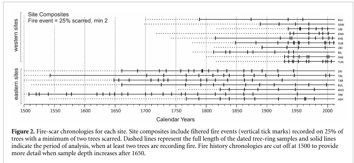
Figure 2. Fire-scar chronologies for each site. Site composites include filtered fire events (vertical tick marks) recorded on 25% of trees with a minimum of two trees scarred. Dashed lines represent the full length of the dated tree-ring samples and solid lines indicate the period of analysis, when at least two trees are recording fire. Fire history chronologies are cut off at 1500 to provide more detail when sample depth increases after 1650.
