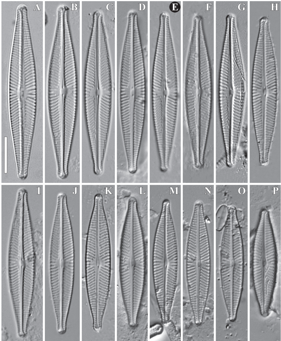
Figure 1. A–P Navicula winoniformis Chudaev, Glushchenko, Kulikovskiy & Kociolek, sp. nov. LM, DIC. Size diminution series. Vietnam, slides no 00269 (A), 00318 (L, P, N), 00323 (I), 00326 (C), 00328 (B), 02079 (O), 03572 (E, F, H, K, M), 03773 (D), 04853 (J). Laos, slide no 00956 (G). Holotype (E). Scale bar: 10 \mu m.
