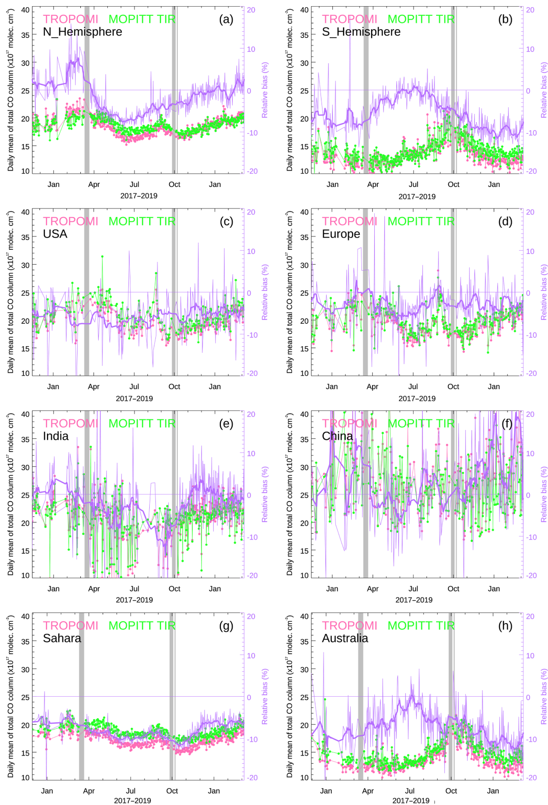
Figure 3. Comparison of collocated land retrievals from TROPOMI (pink) and MOPITT TIR (green) for each ROI analyzed. Filled circles show the daily mean. Thin purple lines indicate the daily relative bias (i.e., accuracy) between the two datasets, and thick purple lines are an 11 d smoothed version with high-frequency variability removed. Gray bars show periods without MOPITT measurements because of hot calibrations (March and October 2018) or a safe-mode maneuver (October–November 2018).
