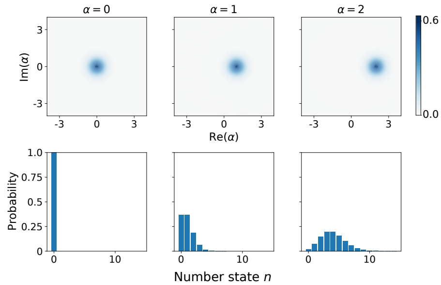
Figure 2.4: Wigner functions and corresponding number state populations of coherent states with \alpha = 0, 1, \text{ and } 2 . From the Wigner functions, one can see that the coherent states correspond to a ground state Wigner function that is displaced by amount \alpha in phase space. The population follows a Poissonian distribution with the average \bar{n} = |\alpha|^2 .
