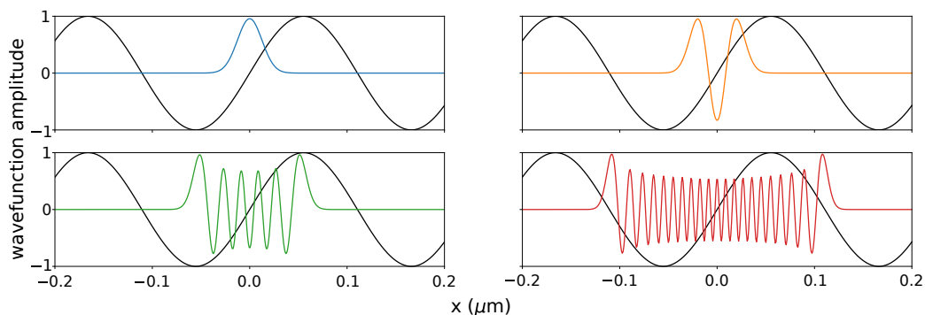
Figure 3.6: Spatial wavefunction (shown in colors) extent in a \omega_0 = 2\pi \times 7 MHz oscillator mode for {}^9\text{Be}^+ compared with Raman laser effective wavelength 2\pi/\Delta k , with \lambda_1 \simeq \lambda_2 313 nm and a 90 degree angle between k_1 and k_2 for number states a) n = 0 , b) n = 2 , c) n = 10 , and d) n = 40 . a) and b) For small spatial wavefunction extent compared with the wavelength, the laser intensity pattern can be approximated to be linear across the ion's wavefunction (Lamb-Dicke approximation). c) and d) As the number state increases, the wavefunction becomes more extended, so the ion sees more of the sinusoidal intensity pattern of the Raman field, and this approximation no longer holds.
