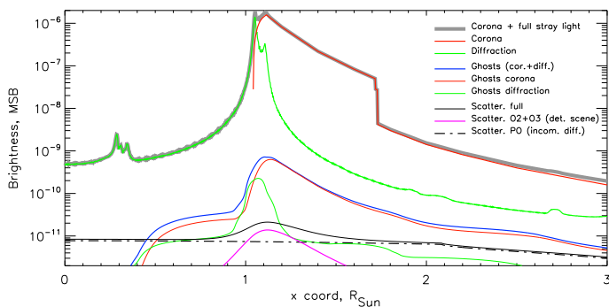
Fig. 12. Radial profiles of the intensity of the coronal light, the diffraction, ghost, and scattered light contributions. The thick red line corresponds to the corona, the thick green line corresponds to the diffraction, and the thick gray line corresponds to the full signal on the detector. The dark blue line represents ghosts of the full image, the thin red and green lines are contributions due to coronal ghosts and diffracted light ghosts. The thin black line shows full scattering light, the dot-dashed line and magenta line show contribution from the primary objective (dot-dashed) and the O2 and O3 lenses (magenta line).
