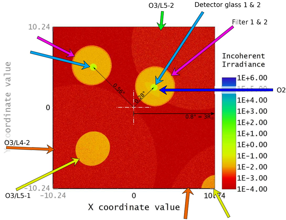
Fig. 3. Image on the detector produced in Zemax OpticStudio in non-sequential regime with two input beams tilted at 0.28^\circ and 0.56^\circ . The white cross denotes the optical axis (center of the FOV), the input beams are marked with thin black arrows, color arrows show ghost contributors produced by the backreflection from the detector and particular optical surfaces. Annotated color arrows correspond to the ghosts, produced by the 0.28^\circ input beam, and the rest correspond to the ghosts produced by the 0.56^\circ beam.
