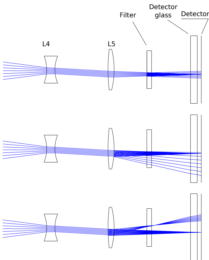
Fig. 4. Ray paths produced by an incoming beam and a ghost beam, formed by the detector and one of the optical surfaces. The incoming beam is backreflected from the detector, travels back almost the same way, experience ghost reflection and travels back forming different path. Top panel shows ray paths produced by the filter, middle panel – by the rear surface of the O3/L5 lens, bottom panel – by the front surface of the O3/L5 lens.
