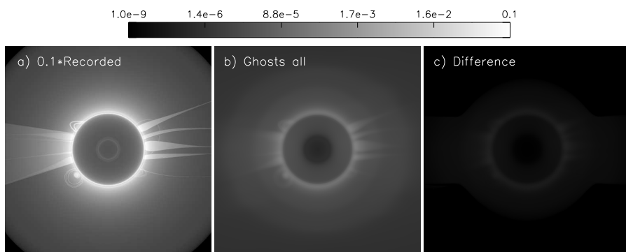
Fig. 9. Analysis of the removal procedure for the synthetic coronal image. Left panel: recorded image \mathbf{R} = \mathbf{I} + \mathbf{G}(\mathbf{I}) ; middle panel: ghost image \mathbf{G}(\mathbf{R}) ; right panel: difference \mathbf{I} - \mathbf{C} between the initial image and the cleared image. Color scale is normalized to the intensity of the recorded image. The intensity in panel (a) is divided by 10 for the visualisation purposes.
