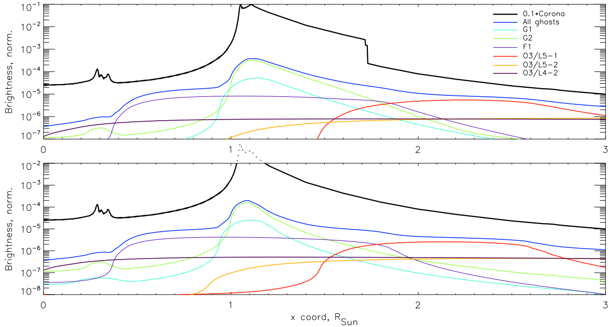
Fig. 8. Radial profiles of the intensity of the synthetic coronal image and various ghost contributions. The upper panel corresponds to the westward equatorial direction in Fig. 7a that crosses the equatorial streamer and the quiet Sun region, the lower panel corresponds to the northward equatorial direction in Fig. 7a that crosses a polar quiet Sun region. In both panels black solid lines show the corona and diffraction (intensity is divided by 10), dark blue lines show the sum of all ghost contribution, other colored lines show contributions from various optical surfaces.
