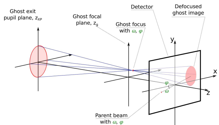
Fig. 5. A sketch representing geometry of the defocused image of a ghost. Configuration of the parent beam and the defocused image correspond to the O3/L5-1 lens surface.
