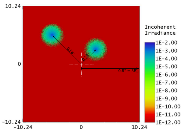
Fig. 11. Image on the detector produced in Zemax OpticStudio in non-sequential regime with scattering on the O2 lens for the two input beams tilted at 0.28^\circ and 0.56^\circ . The logarithmic color scale corresponds to irradiance and is normalized to the peak irradiance of the scattered images.
