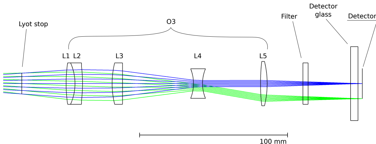
Fig. 2. Detailed optical layout of the rear part of the ASPIICS coronagraph. Blue and green lines denote ray paths propagating along the optical axis (blue) and at the edge of the FOV – 0.8^\circ ( 3R_\odot ) (green).
