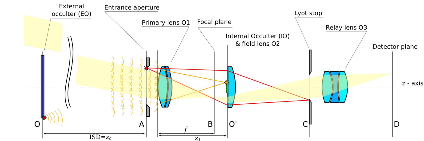
Fig. 1. Functional optical layout of the ASPIICS coronagraph. Dim yellow light represents regular coronal beam, orange arches and lines – light that diffracts on EO, the red lines represent the light diffracted at the entrance aperture.
