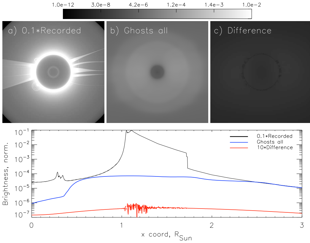
Fig. B.1. Analysis of the removal procedure for the synthetic coronal image with the removed detector glass. The top panels have the same notation as in Fig. 9, the bottom panel shows intensities of R , G(R) and I – C in the westward from the disk center direction.
