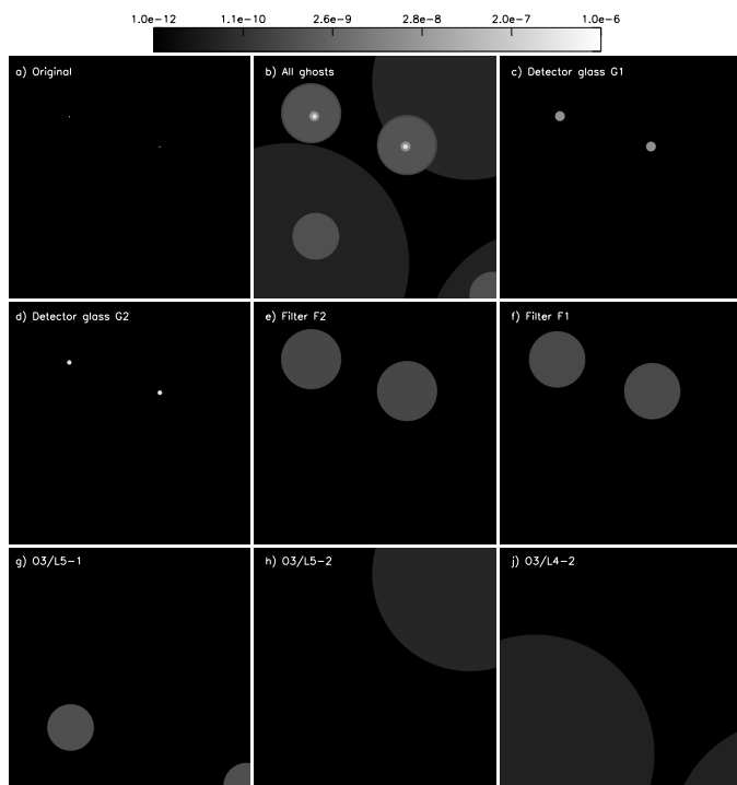
Fig. 6. Ghost images produced for an input image with two bright pixels (up-right and up-left from the center) representing two plane-parallel beams tilted at 0.28^\circ and 0.56^\circ . The panels denote: a) the input image; b) full ghost image; c) ghost image produced by the front surface of the detector glass; d) by the rear surface of the detector glass; e) by the rear filter surface; f) by the front filter surface; g) by the rear surface of the O3/L5 lens; h) by the front surface of the O3/L5 lens; j) by the rear surface of the O3/L4 lens. Logarithmic color scale (shown in the top of the figure) is normalized to the intensities of the input beams.
