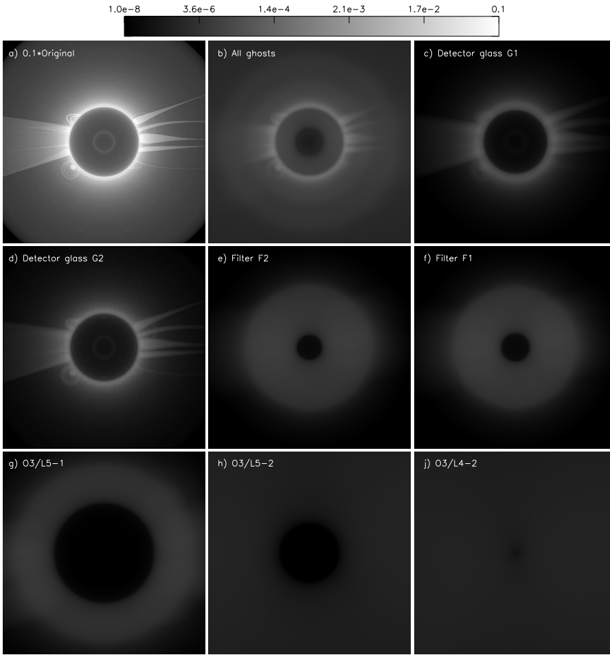
Fig. 7. Ghost images for the synthetic coronal image. Panel (a) shows the input image with coronal and diffracted light superposed, other panels show different ghosts and have the same meaning as in Fig. 6. Color scale is normalized to the intensity of the input image. The intensity in panel (a) is divided by 10 for the visualisation purposes.
