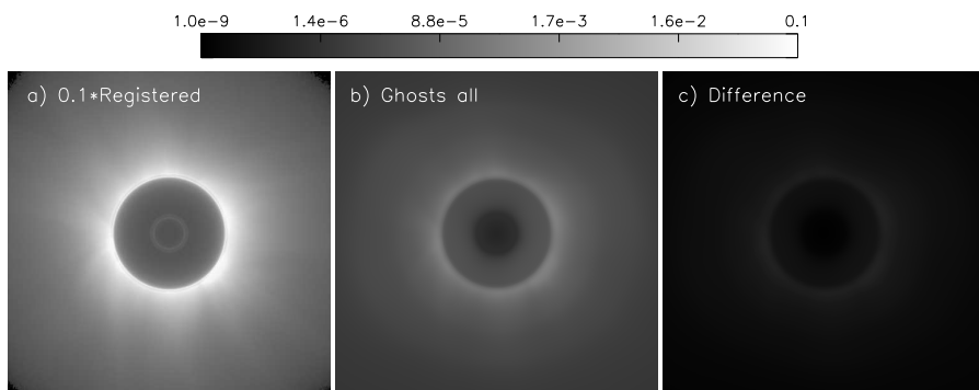
Fig. 10. Analysis of the removal procedure for the coronal image obtained during a total solar eclipse. Panels have the same meaning as in Fig. 9.
