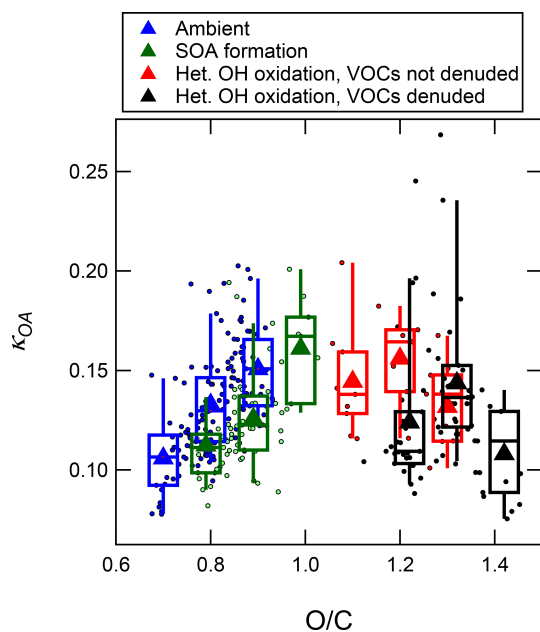
Figure 11. Binned averages of hygroscopicity of OA ( \kappa_{\text{OA}} ) measured at 160 nm as a function of bulk O : C of the OA. The data include ambient data, measurements after 1–3 eq. days OH aging to sample maximum SOA formation, and measurements after 12–44 eq. days aging sampled through (or not through) a gas denuder in order to sample the result of heterogeneous oxidation of preexisting OA.
