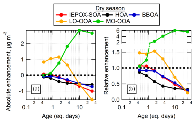
Figure 10. Absolute (a) and relative (b) changes in PMF factors as a function of eq. days of OH aging in the OH-OFR for the dry season. Note that the y axis in (b) is split in order to more clearly show the region below a value of 1.
