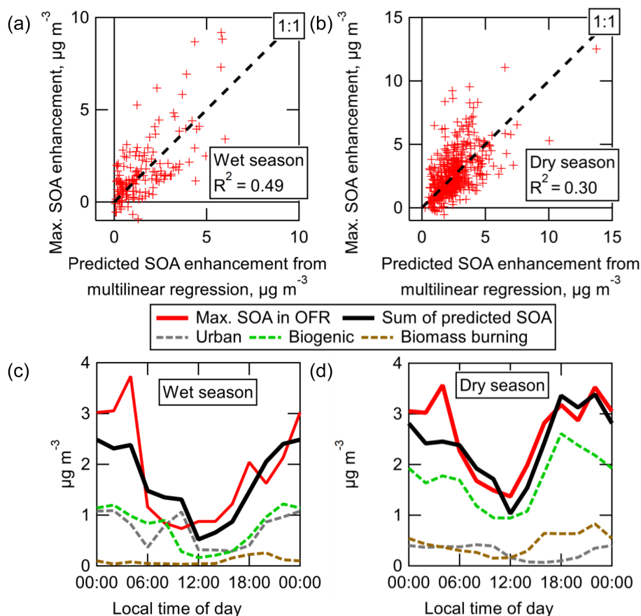
Figure 12. (a, b) Maximum measured SOA enhancement from OH oxidation in the OFR at the T3 site during the wet and dry seasons vs. the total amount predicted from multilinear regression analysis. (c, d) Diurnal average values of the maximum measured SOA formation from OH oxidation during each season, the amount attributed to each emission source, and the total amount predicted from all sources.
