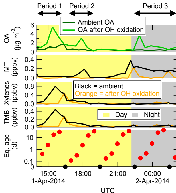
Figure 4. An example of OA concentrations in ambient air and after OH oxidation of ambient air in the OFR at the T2 site, shown together with MT, xylenes, and trimethylbenzene (TMB) measured in ambient air and after OH oxidation. The \text{OH}_{\text{exp}} is also shown (in eq. days). Daytime (nighttime) hours are indicated with the yellow (grey) background. OH age was cycled through a range of exposures, including no added exposure (black circles) where none of the VOCs were reacted in the OFR. This example illustrates how SOA formation in the OFR can come from urban (Period 1), biogenic (Period 3), or mixed (Period 2) precursors, depending on ambient conditions.
