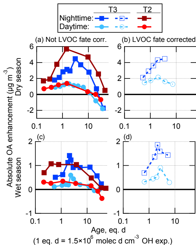
Figure 5. Absolute OA enhancement after OH oxidation in the OFR as a function of photochemical age, shown as binned averages for the wet (c, d) and dry (a, b) seasons at both the T2 and T3 measurement sites, and split into daytime (06:00–18:00 LT) and nighttime (18:00–06:00 LT) data. These data are shown both not corrected (left) and corrected (right) for LVOC fate. Note that the scale of the y axis is different between the wet and dry season panels. The average ambient OA concentrations during the measurement times used here were 1.2 and 6.9 \mu\text{g m}^{-3} at T2 in the wet and dry seasons, and 1.3 and 9.5 \mu\text{g m}^{-3} at T3 in the wet and dry seasons, respectively.
