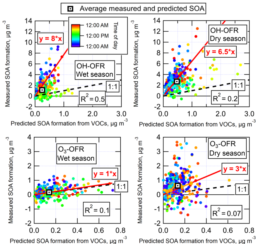
Figure 8. Measured SOA formation vs. the concentration of SOA predicted to form from the oxidation of ambient VOCs, shown for OH and O 3 oxidation during both wet and dry seasons. Regression lines, correlation coefficients, and average measured and predicted SOA are shown for each OFR type and season. Standard errors of the mean of all average measured and predicted SOA values were smaller than the size of the marker and are thus not shown. Data are colored by local time of day. Measured SOA formation is corrected for LVOC fate.
