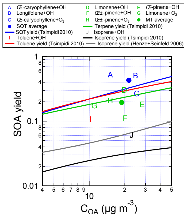
Figure 7. SOA yields measured for individual VOCs in the OFR by standard addition into ambient air, as a function of OA concentration. Typical SOA yield parameterizations (derived from a chemical transport model, which was informed using environmental chamber experiments; Lane et al., 2008a, b; Tsimpidi et al., 2010) are also shown. The VOCs were injected into ambient air at the entrance to the OFR, and aged between 0 and 5 eq. days. Data are corrected for LVOC fate.
