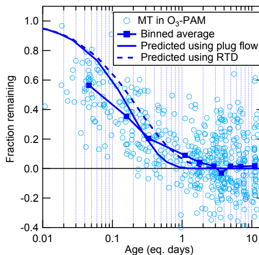
Figure 2. Fraction of ambient MT remaining after \text{O}_3 oxidation in the OFR, as a function of photochemical age. Binned averages of the fraction remaining are also shown, compared to the amount predicted to remain assuming either plug flow or using the RTD of particles from Lambe et al. (2011a).
