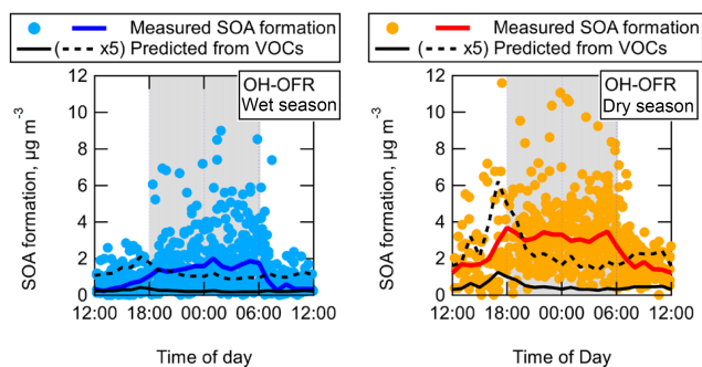
Figure 9. Measured SOA formation vs. local time of day and mean diurnal cycles of measured and predicted SOA formation, shown for OH oxidation during both wet and dry seasons. For clarity, the predicted SOA from ambient VOCs is also shown multiplied by 5 for easier comparison of the trend relative to measured SOA formation.
