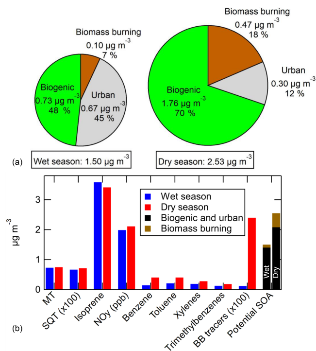
Figure 13. (a) The amounts and fraction of the total SOA formation from OH oxidation in the OFR at the T3 site that were attributed to biogenic, urban, and biomass burning emission types using multilinear regression analysis. (b) Comparison of the average tracer concentrations and potential SOA formation during wet and dry seasons.
