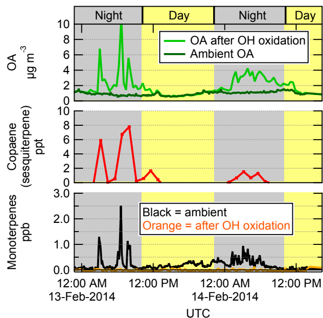
Figure 3. An example of the time series of OA concentrations measured in ambient air and after OH oxidation of ambient air in the OFR at the T3 site, shown together with ambient copaene (a sesquiterpene, measured by SV-TAG) and monoterpenes (measured by PTR-TOF-MS before and after the OFR). Daytime (nighttime) hours are indicated with the yellow (grey) background. \text{OH}_{\text{exp}} in the OFR was held constant throughout this time at approximately 3 eq. days. The SOA formed in the OFR is shown as measured, without the LVOC fate correction. In this example, the SOA formation from OH oxidation closely follows the availability of ambient biogenic gases, though the amount of SOA formed was substantially larger than could be formed from the measured ambient gases (see Sect. 3.5).
