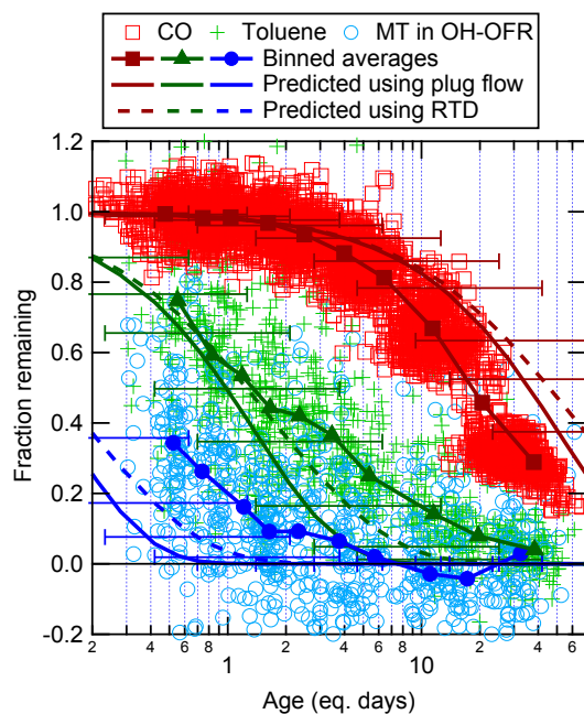
Figure 1. Fraction of ambient toluene, ambient MT, and injected CO remaining after OH oxidation in the OFR, as a function of equation-estimated photochemical age (Peng et al., 2015). Binned averages of the fraction remaining are also shown, compared to the amount predicted to remain assuming either plug flow or using the residence time distribution (RTD) of particles from Lambe et al. (2011a). Factor-of-3 error bars are shown for the prediction using RTD, representing the uncertainty in the model-derived \text{OH}_{\text{exp}} estimation equation (Li et al., 2015; Peng et al., 2015).
