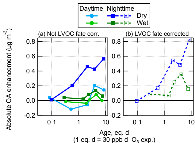
Figure 6. Absolute OA enhancement after \text{O}_3 oxidation in the OFR as a function of photochemical age, shown as binned averages for the wet and dry seasons at the T3 measurement site, and split into daytime (06:00–18:00 LT) and nighttime (18:00–06:00 LT) data. These data are shown both not corrected (a) and corrected (b) for LVOC fate.
