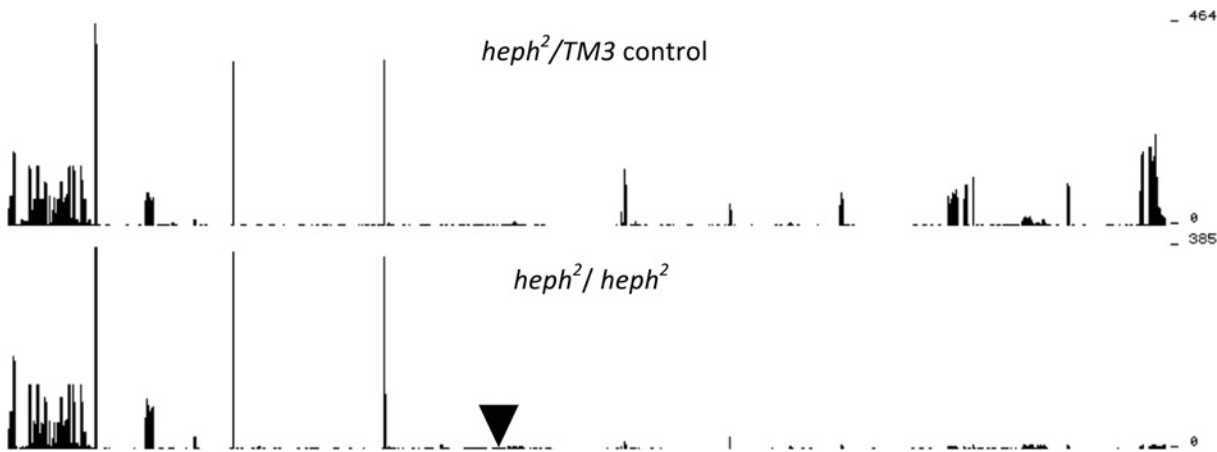
Fig 1. Loss of RNA-Seq coverage in the heph 2 homozygous mutant in the 3' portion of the heph gene, downstream of the P element insertion site. The control sample is shown on the top graph and the heph 2 homozygous mutant on the bottom graph. The inverted triangle represents the location of the P element insertion in an intron (intron has been condensed to save space). There are two transcription start sites for the dmPTB or heph locus, producing transcripts with proximal and distal 5'UTRs. The abundant male germline-specific transcript, which is disrupted in the heph 2 mutant, results from the use of the distal or upstream promoter. The P element in heph 2 is inserted into an intron corresponding to the transcript with distal 5' UTR. However, for the heph 03429 mutant, showing embryonic lethality, the P element is inserted into an intron downstream of the proximal 5' transcript start site. This transcript start site is relevant for the non-sex-specific, including embryonic, function of dmPTB ; no reads were found that spanned the other end of the P element insertion into the heph gene [26].
