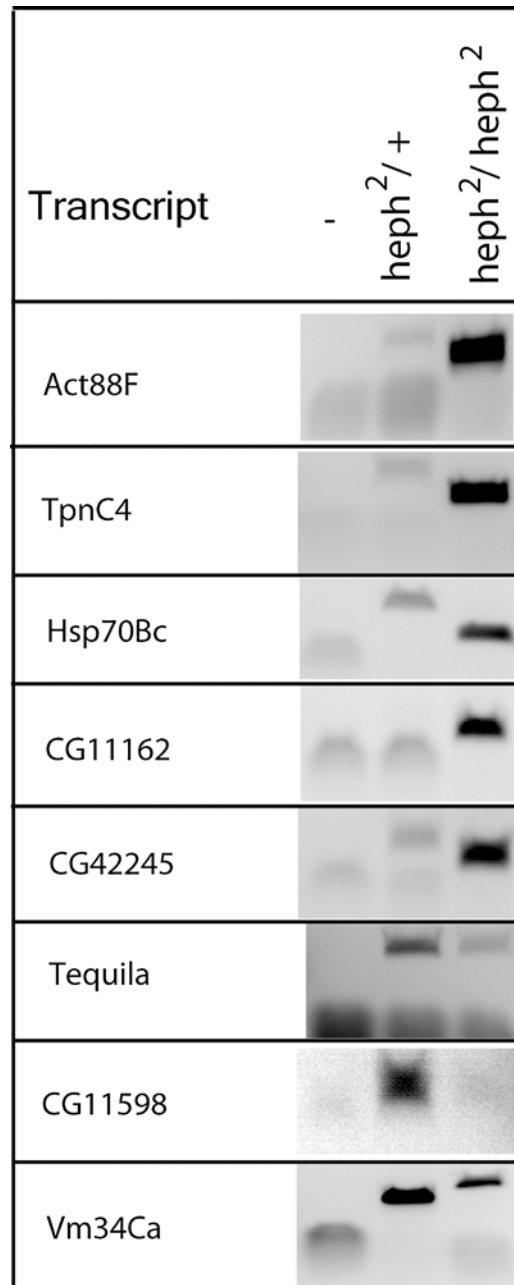
Fig 3. RT-PCR analysis reveals differentially expressed transcripts. RNA from the wild type control and the heph 2 mutant was analyzed by RT-PCR analysis. Gene-specific primer pairs were used for amplification of several randomly picked genes that showed significant differential expression. For Tequila , primer pairs were designed to test alternative 5' ends (transcription start site usage).
