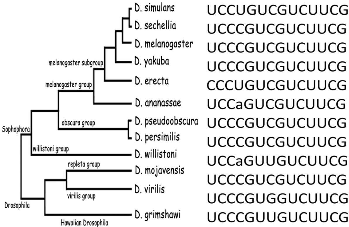
Fig 6. Identification of a conserved PTB binding site in Mlc1 . Putative PTB binding site in Mlc1 conserved in 12 Drosophila species is shown. The highest affinity SELEX sequence that binds PTB in vitro is shown for comparison.
