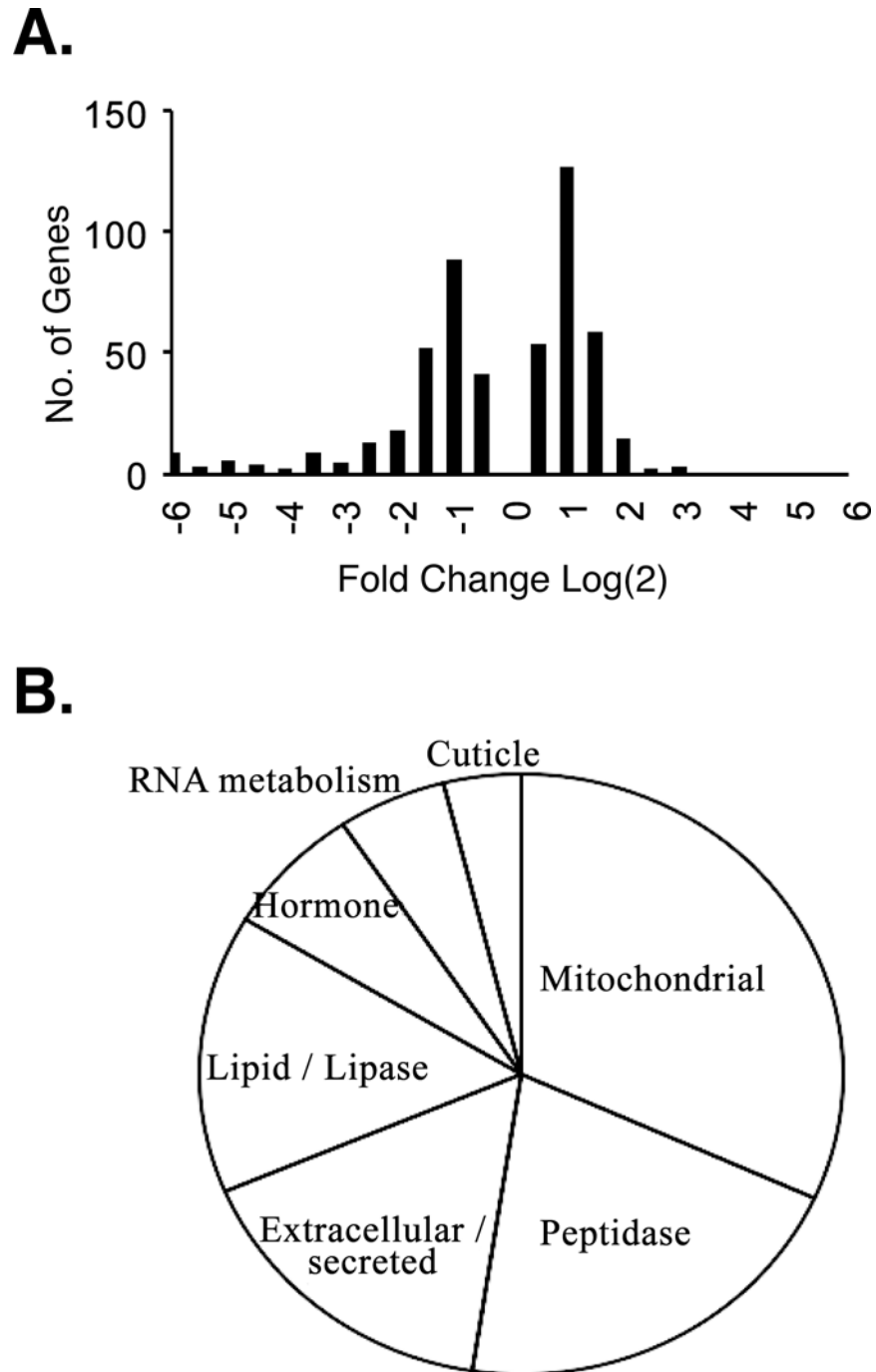
Fig 2. Effect of the heph 2 mutation on fold-changes in gene expression. Histogram of fold-changes in the heph 2 mutants of genes called significant by Cufflinks (note that Cufflinks did not call any genes significant below 0.78 log 2 change). The list is provided in S1 Table . (B). Pie chart representing gene ontology categories over-represented in the genes that are significantly affected in the heph 2 mutant.
