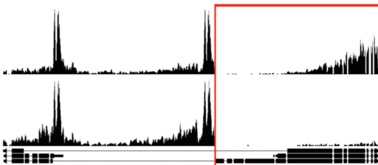
Fig 4. Use of alternative transcription start sites in the heph 2 mutant. (A) RNA Seq read pileup across a Paramyosin alternative transcription start site, where alternative transcription start sites highlighted by the box. (B) RNA Seq read pileup across a Tequila alternative transcription start site, where the 5' end showing the most difference is highlighted by the box. For RT-PCR validation of Tequila alternative transcription start site usage, see Fig 3.
