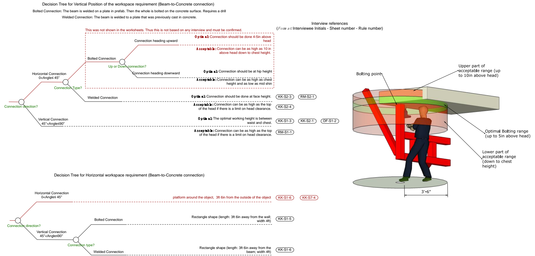
FIGURE 7: Decision tree for a Beam-to-Concrete connection
