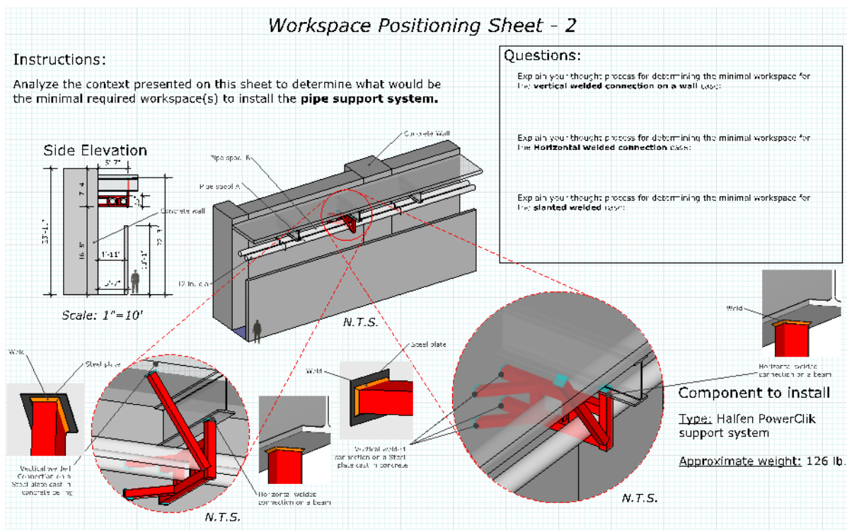
FIGURE 2: A sample worksheet describing a piping support system welded to a beam and to a concrete wall. (Note, the connection points are highlighted in cyan.)
