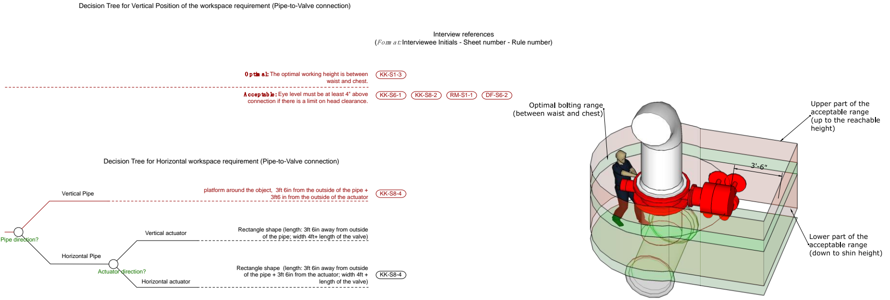
FIGURE 9: Decision tree for a valve-to-pipe connection
