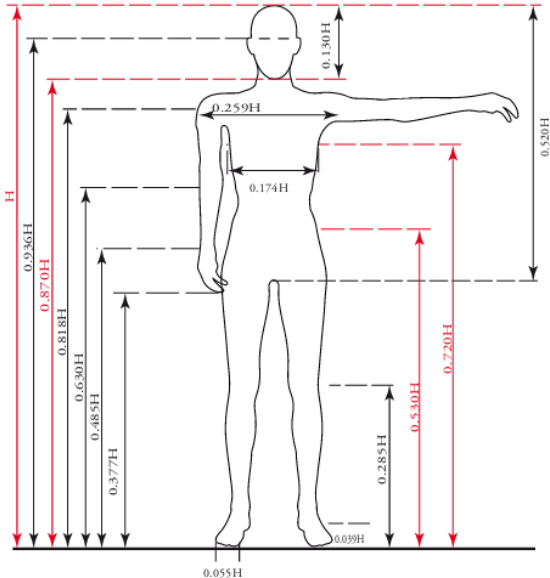
FIGURE 4: Body segment parameters, from (Drillis and Contini, 1966) (The parameters used in this study are highlighted in red.)
