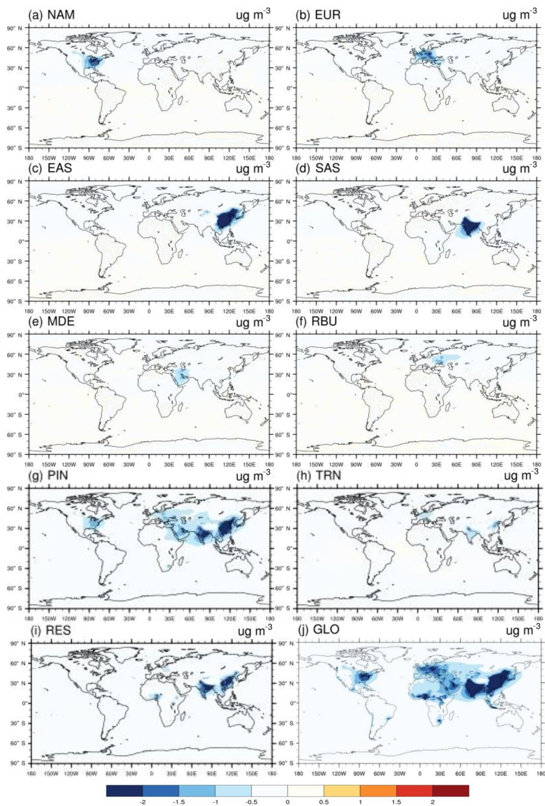
Figure 2. Global difference in multi-model annual mean \text{PM}_{2.5} concentrations ( \mu\text{g m}^{-3} ) in 20% emission reduction scenarios relative to the baseline for the year 2010 in (a) North America (NAM), (b) Europe (EUR), (c) East Asia (EAS), (d) South Asia (SAS), (e) the Middle East (MDE), and (f) Russia–Belarus–Ukraine (RBU), the (g) power and industry (PIN), (h) transportation (TRN), and (i) residential (RES) sectors, and (j) globally (GLO).
