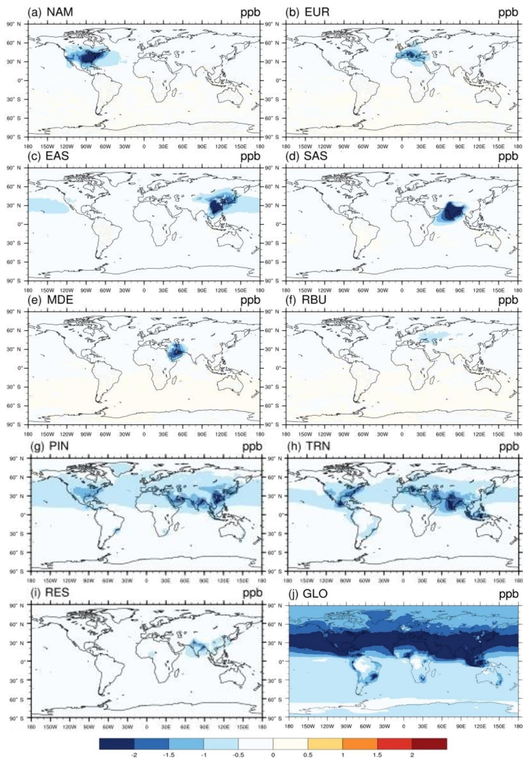
Figure 1. Global difference in multi-model mean \text{O}_3 concentrations (ppb) in 20% emission reduction scenarios relative to the baseline for the year 2010 in (a) North America (NAM), (b) Europe (EUR), (c) East Asia (EAS), (d) South Asia (SAS), (e) the Middle East (MDE), and (f) Russia–Belarus–Ukraine (RBU), the (g) power and industry (PIN), (h) transportation (TRN), and (i) residential (RES) sectors, and (j) globally (GLO), shown for the 6-month \text{O}_3 season average of 1 h daily maximum health-relevant metric.
