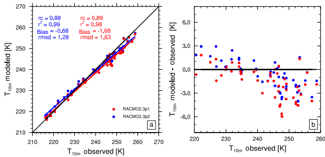
Figure 5. (a) RACMO2.3p2 (blue) and RACMO2.3p1 (red) and (b) modelled minus observed 10 m snow temperature as a function of the 10 m snow temperature observations. Denoted are the slope, determination coefficient r^2 , bias and root mean square deviation (RMSD) for both model versions.
