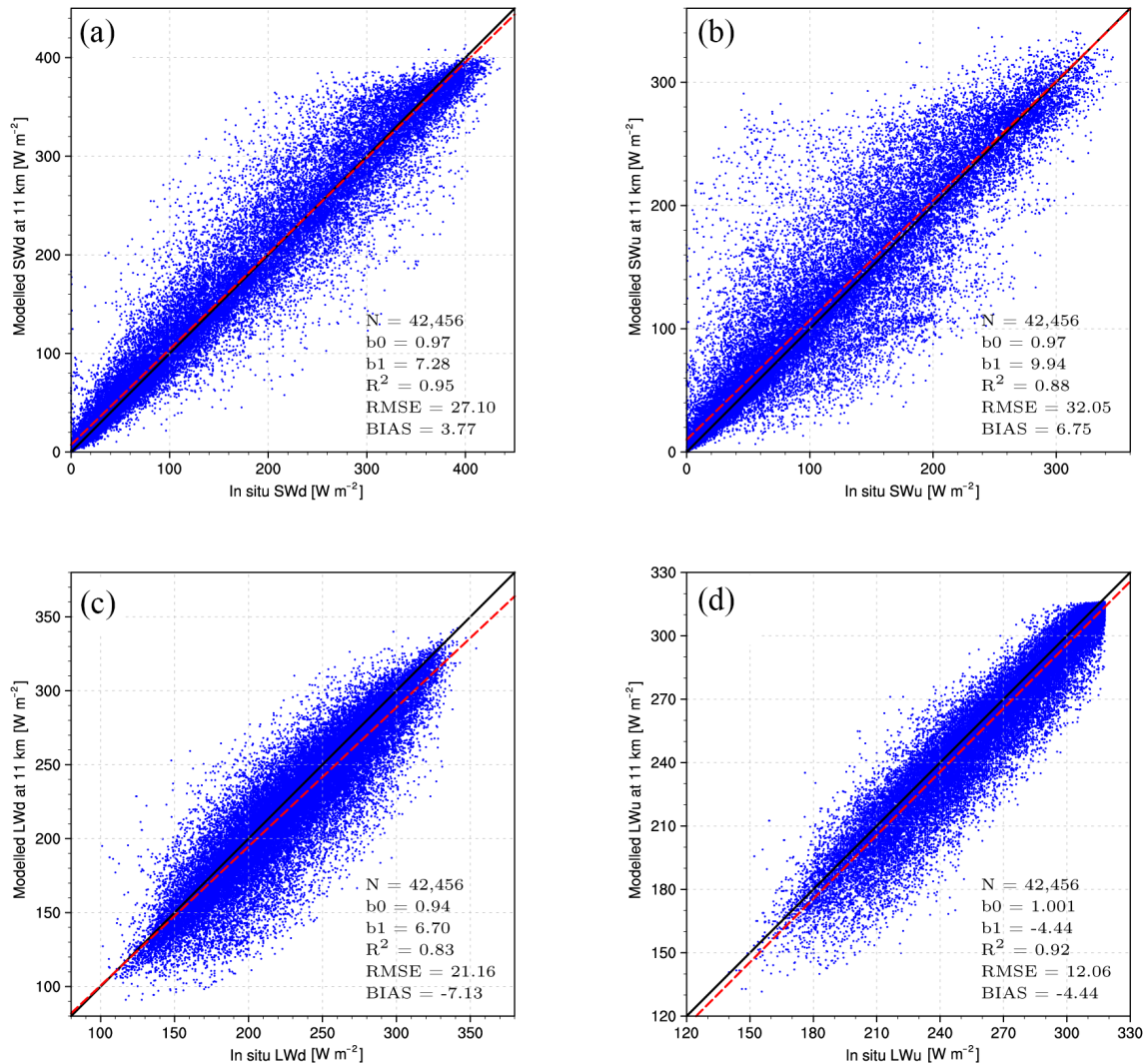
Figure 4. Comparison between daily average modelled (RACMO2.3p2, 2004–2016) and observed (a) shortwave downward, (b) shortwave upward, (c) longwave downward and (d) longwave upward radiation ( \text{W m}^{-2} ) collected at 23 AWSs (green dots in Fig. 1). For each variable, a regression including all records is displayed as a red dashed line. Statistics including number of records ( N ), the linear regression slope ( b_0 ) and intercept ( b_1 ), determination coefficient ( R^2 ), bias and RMSE are listed for each variable.
