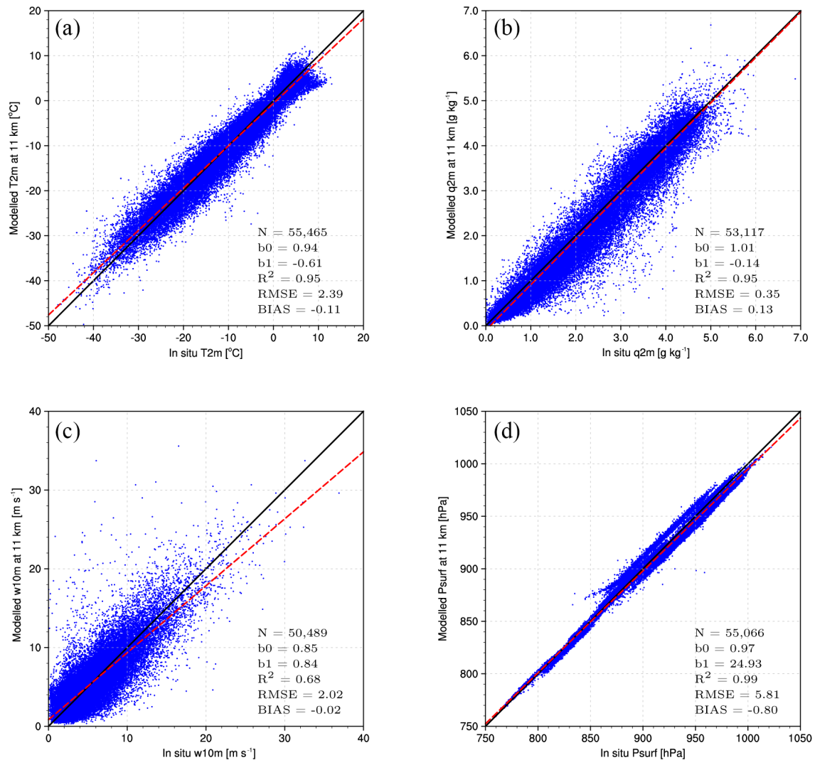
Figure 3. Comparison between modelled (RACMO2.3p2, 2004–2016) and observed (a) 2 m temperature ( T_{2m} , °C), (b) 2 m specific humidity ( q_{2m} , g kg -1 ), (c) 10 m wind speed ( w_{10m} , m s -1 ) and (d) surface pressure ( P_{surf} , hPa) collected at 23 AWSs (green dots in Fig. 1). For each variable, the linear regression including all records is displayed as a red dashed line. Statistics including number of records ( N ), regression slope ( b_0 ) and intercept ( b_1 ), determination coefficient ( R^2 ), bias and RMSE are listed for each variable.
