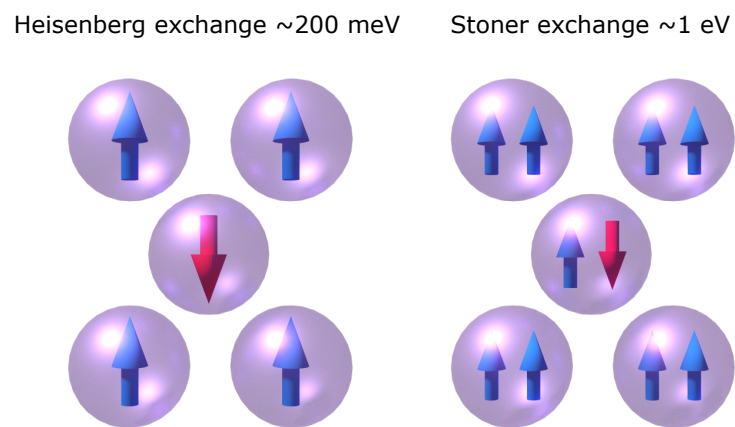
Figure 2.8: Exchange in the Stoner and Heisenberg models. In the Heisenberg model (left), the exchange energy corresponds to a reversal of a local magnetic moment in the mean exchange field of other moments. In the Stoner model, it corresponds to a spin flip of a single electron in the sea of all other electrons.
