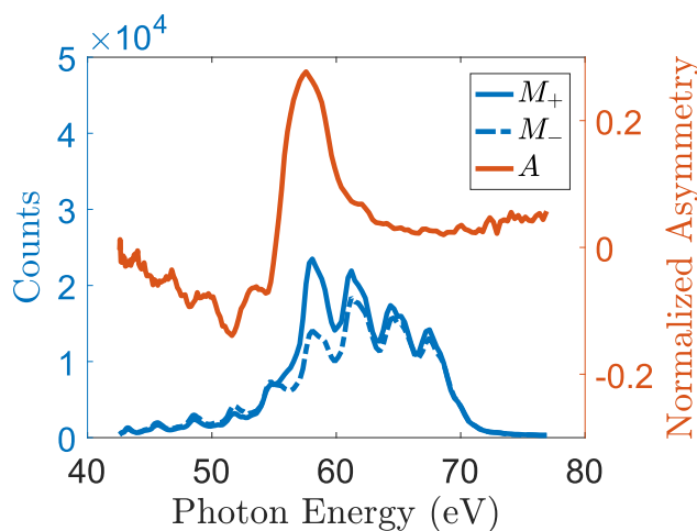
Figure 4.1: An example T-MOKE asymmetry spectrum (orange) at the M -edge of Co. The HHG spectra reflected from the sample when it was positively (solid) and negatively (dashed) magnetized are shown in blue.
