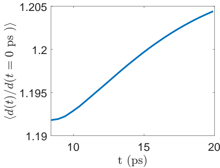
Figure 6.21: Calculated time-dependent domain wall width changes relative to the static case.
