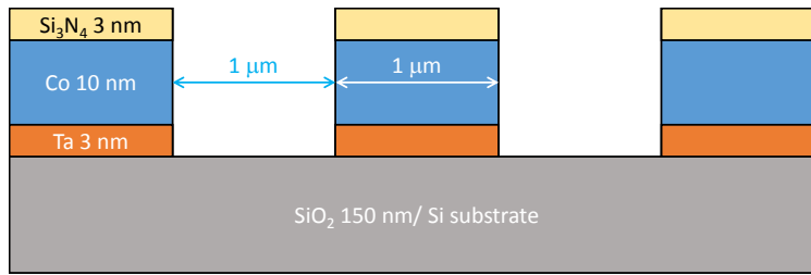
Figure 4.11: Sample structure for angle-resolved T-MOKE. A 10 nm Co film is grown on a Si wafer with a 3 nm Ta seed layer and a 3 nm Si 3 N 4 cap. The sample was lithographically patterned to form a 500 lines/mm grating.
