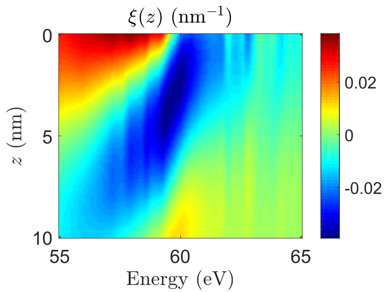
Figure A.2: T-MOKE EUV depth sensitivity function of a 10 nm Co film with a multilayer composition of \text{SiO}_2 (150 nm)/Co (10 nm)/ \text{GeO}_2 (3 nm) at a 52^\circ incidence. The magneto-optical Voigt parameter Q was taken from Ref. [168].
