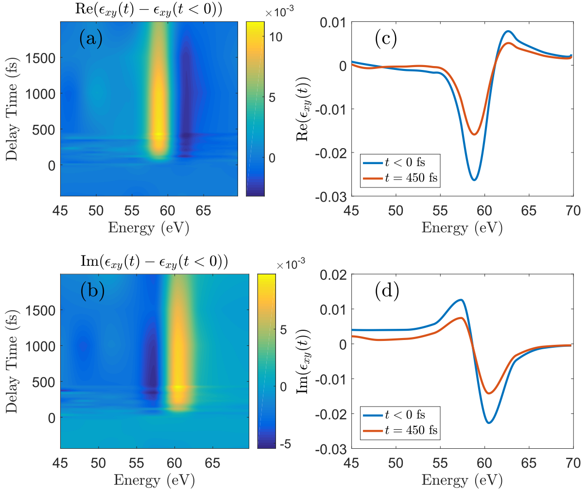
Figure 4.20: Transient changes in \epsilon_{xy} measured with time-resolved D-MOE: (a) \text{Re}(\Delta\epsilon_{xy}(E, t)) = \text{Re}(\epsilon_{xy}(E, t) - \epsilon_{xy}(E, t < 0)) , (b) \text{Im}(\Delta\epsilon_{xy}(E, t)) = \text{Im}(\epsilon_{xy}(E, t) - \epsilon_{xy}(E, t < 0)) . Also shown is a comparison of the (c) real and (d) imaginary parts of \epsilon_{xy} at the time of maximum demagnetization t = 450 fs with the unperturbed state at t < 0 .
