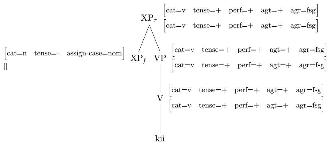
Figure 5.9: Elementary tree for light verb kar 'do' inflected as kii 'do.fem.sing.perf'
